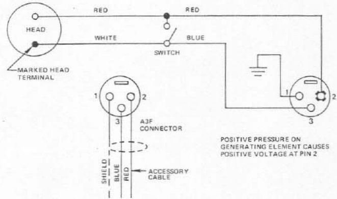
FIGURE 2 – Wiring Diagram
