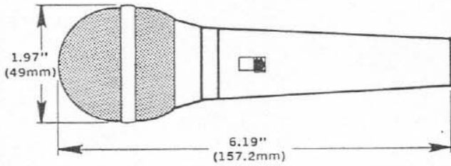
FIGURE 1 – Dimensions
