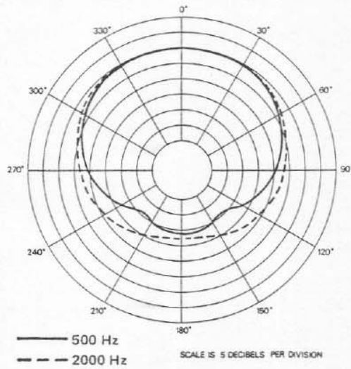
FIGURE 4 – Polar Response
