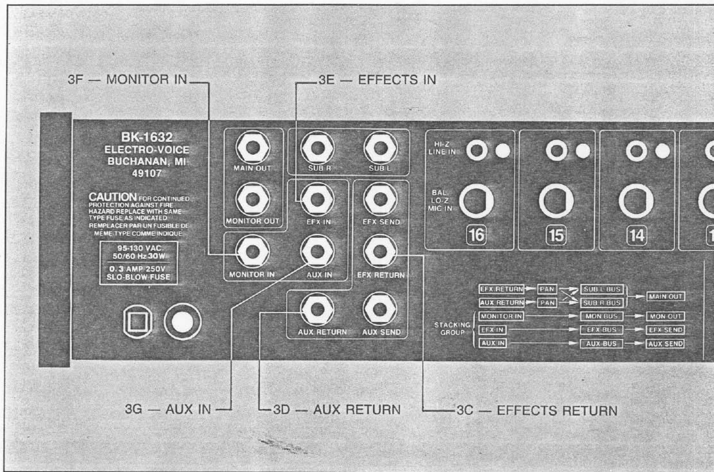
FIGURE 3 — Input Jacks
