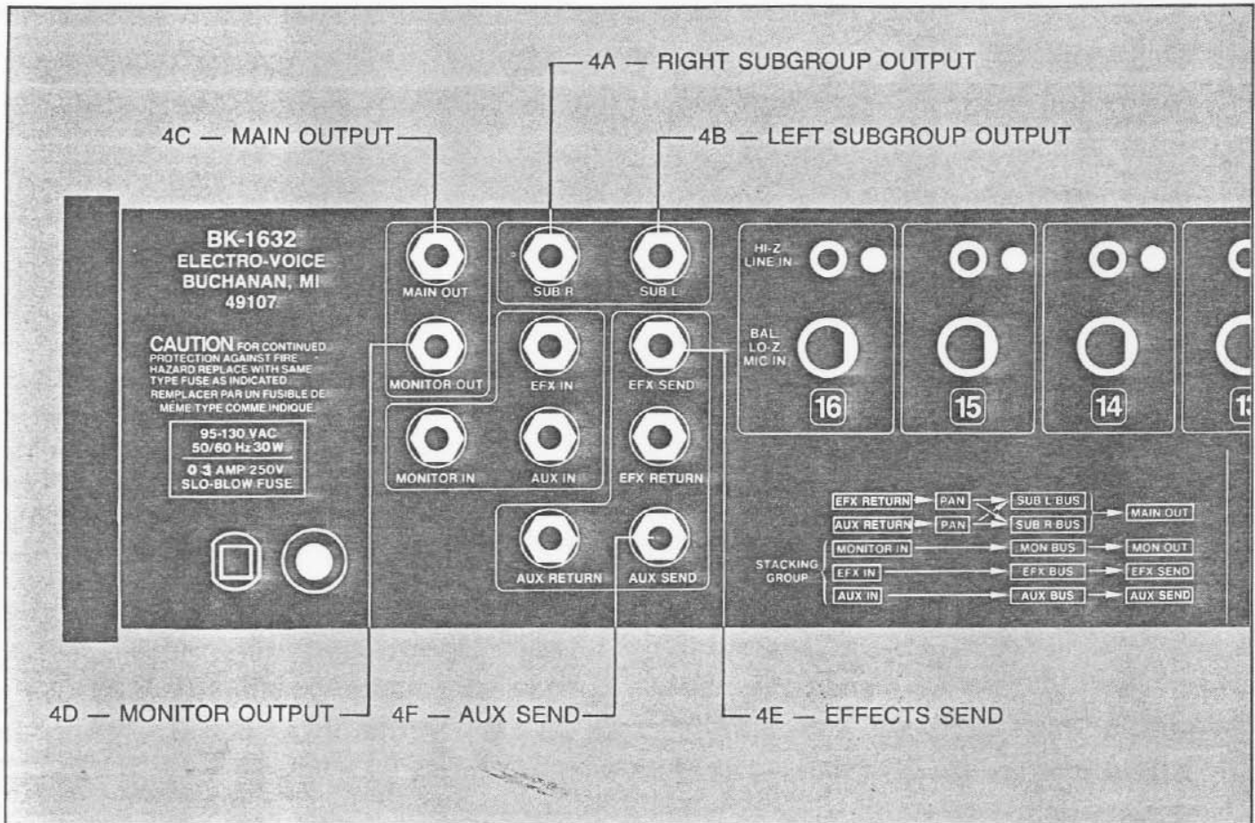
FIGURE 4 — Output Jacks
