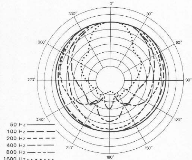
FIGURE 4 – TL505/DL18X Polar Response 4 V RMS of Octave-Band-Limited Pink Noise in Anechoic Environment, 10 Ft on Axis in Horizontal Plane (5 dB per division)
