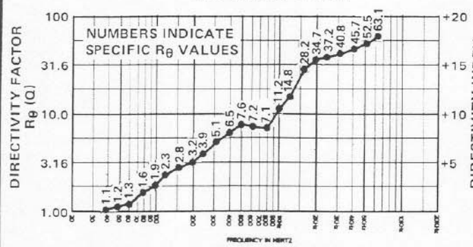
FIGURE 6 – TL505/DL18X Directivity Factor and Directivity Index vs. Frequency
