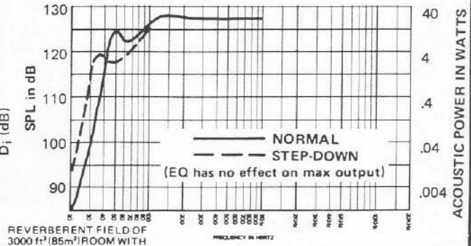
FIGURE 7 TL505/DL18X Theoretical Low-Frequency Maximum Acoustic Output vs. Frequency
