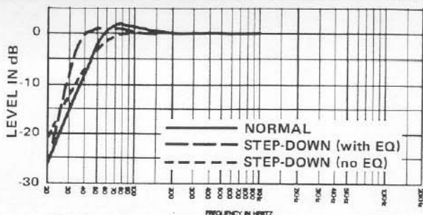
FIGURE 2B – Bass Response in 7.1-Ft 3 Enclosure (TL505)
