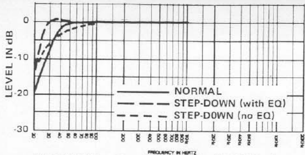
FIGURE 2A – Bass Response in 13-Ft 3 Enclosure (TL405)
