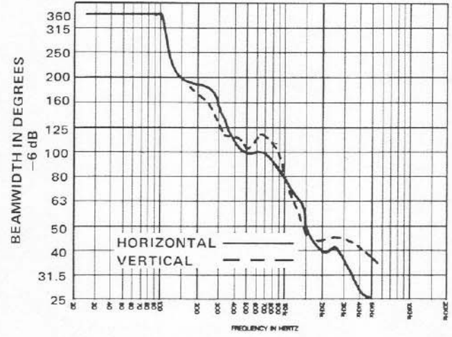
FIGURE 5 TL505/DL18X Beamwidth vs. Frequency
