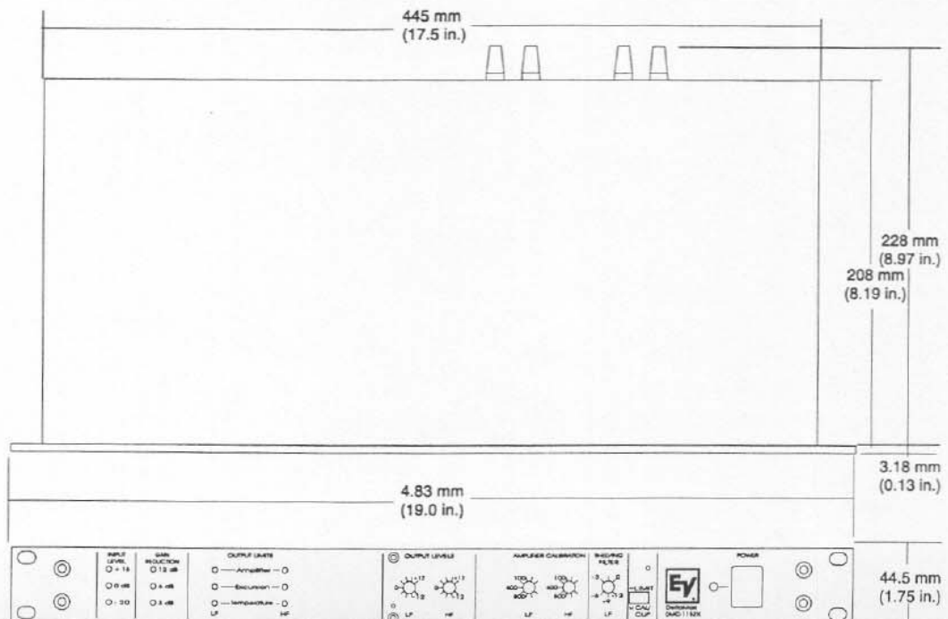
Figure 4—DMC-1152X Dimensions
