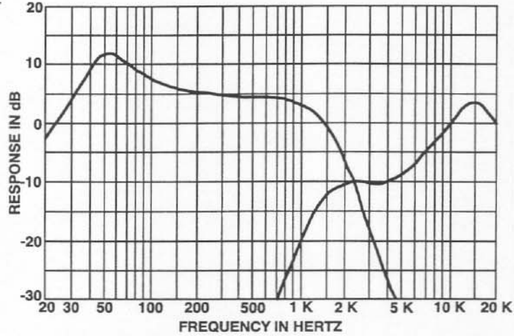
Figure 2—DMC-1152X Frequency Response
