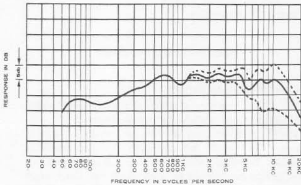
Figure 1—Representative Frequency Response and Range of Balance Control Action
