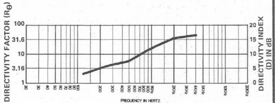
FIGURE 5 — LF118 Directivity Factor and Directivity Index (Derived from Octave Band Horizontal and Vertical Polar Responses)
