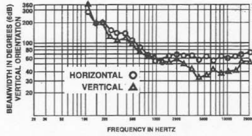
FIGURE 4 — MTH-2.5/64BT Beamwidth vs. Frequency
