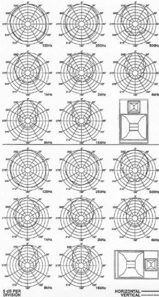
FIGURE 3 — MTH-2.5/64BT Polar Response
