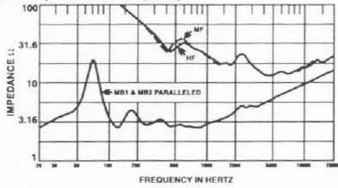
FIGURE 2 — Impedance vs. Frequency
