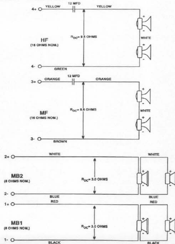
FIGURE 7 — Wiring Diagram
