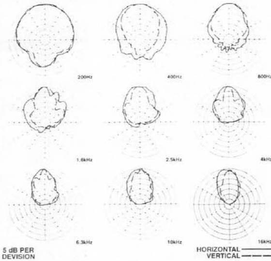
FIGURE 3 — Polar Response
