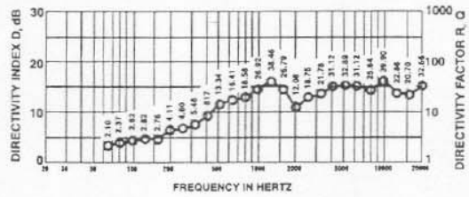
FIGURE 6 — MTH-4.5/64B Harmonic Distortion
