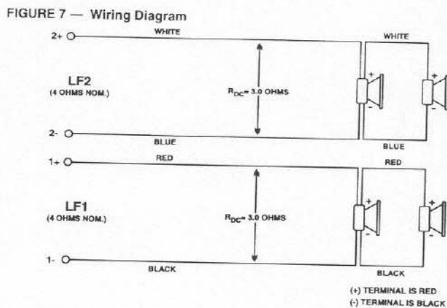
FIGURE 7 — Wiring Diagram
