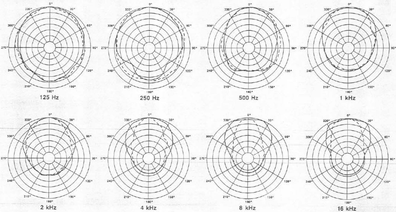
FIGURE 2 — Polar Response
