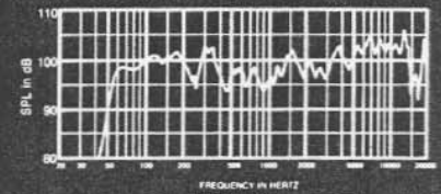
FIGURE 1 MTS-1 Axial Frequency Response 1 Watt/1 Meter
