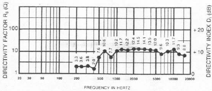
FIGURE 4 Directivity Factor R_D (Q) and Directivity Index ( D_i ) vs. Frequency
