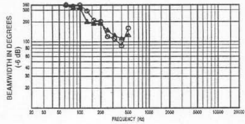
FIGURE 5 — Beamwidth vs. Frequency
