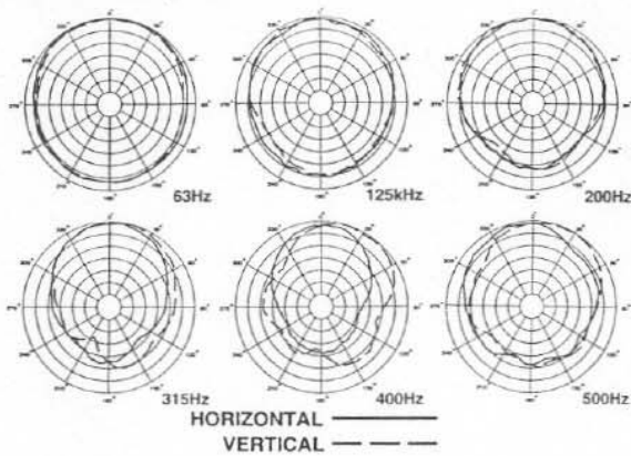
FIGURE 4 — Polar Response
