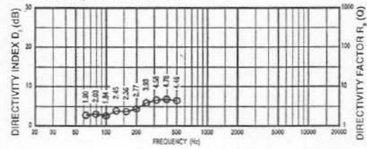
FIGURE 6 — Directivity vs. Frequency
