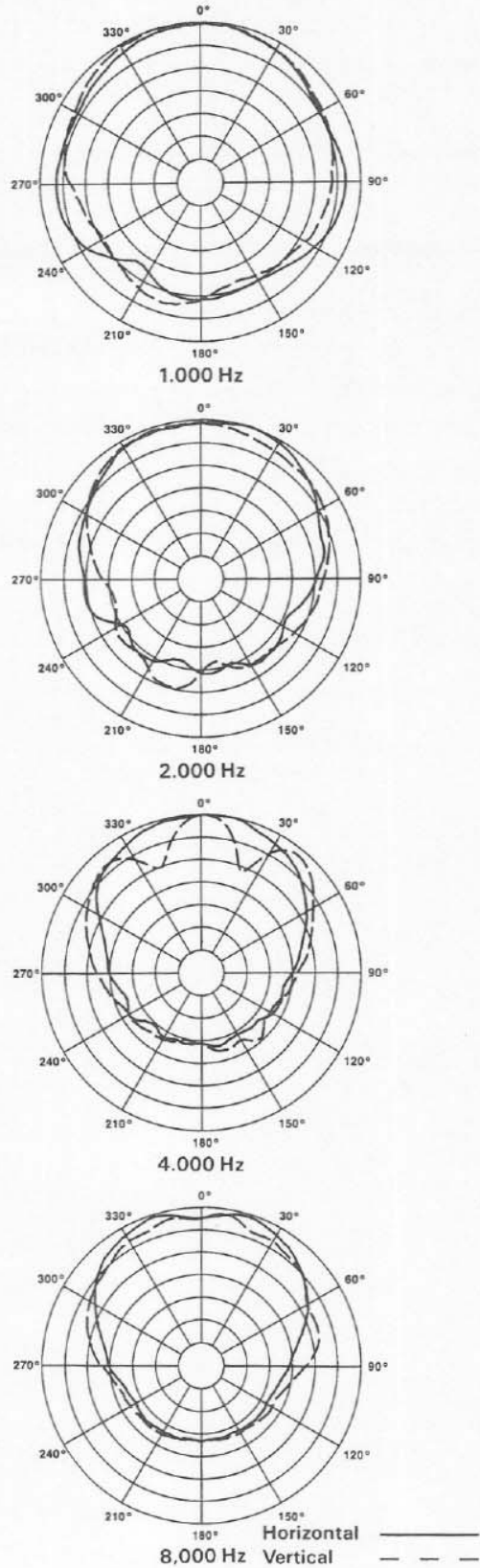
FIGURE — 4 Polar Response
