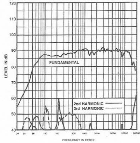
FIGURE 5 — Harmonic Distortion, 0.01 Rated Power Input put (1 watt)
