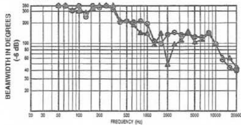
FIGURE 3 — Beamwidth vs. Frequency (whole space anechoic environment)
