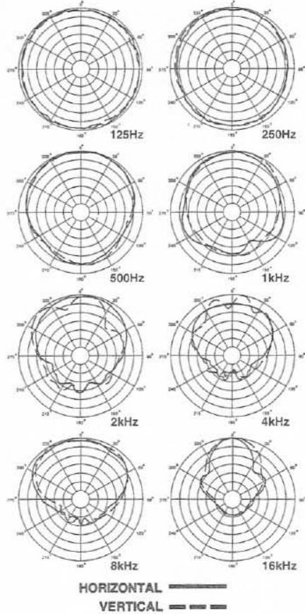
FIGURE 2 — Polar Response
