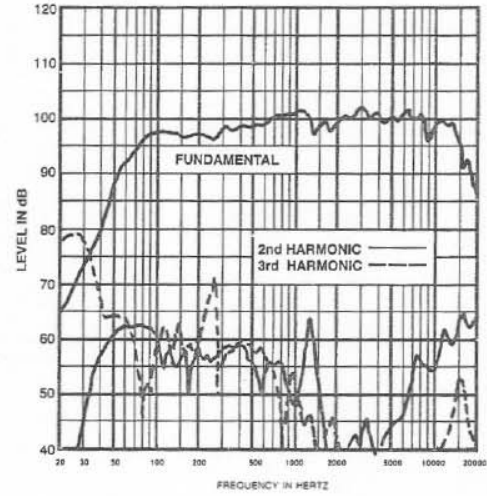
FIGURE 6 — Harmonic Distortion, 0.1 Rated Power Input put (10 watts)
