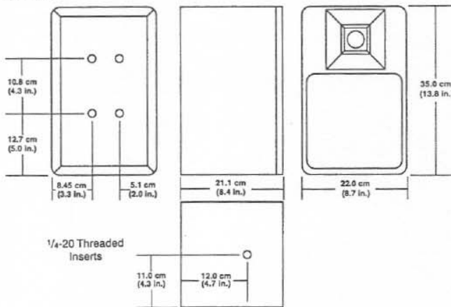
FIGURE 8 — Dimensions
