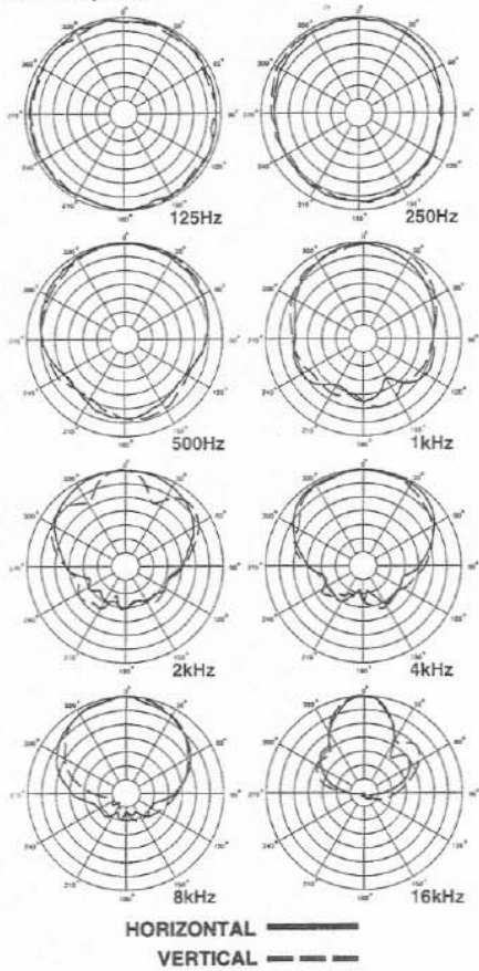
FIGURE 2 — Polar Response
