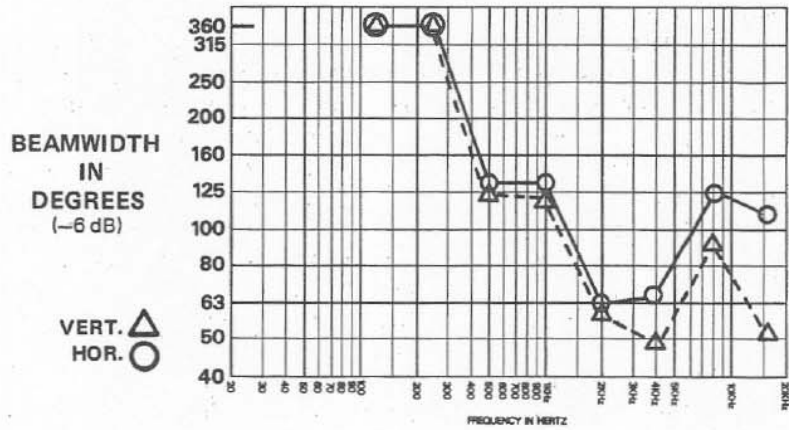
FIGURE 6 – S12-2A Beamwidth vs Frequency (System Long Axis Vertical)
