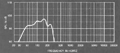
FIGURE 1 — Frequency Response
