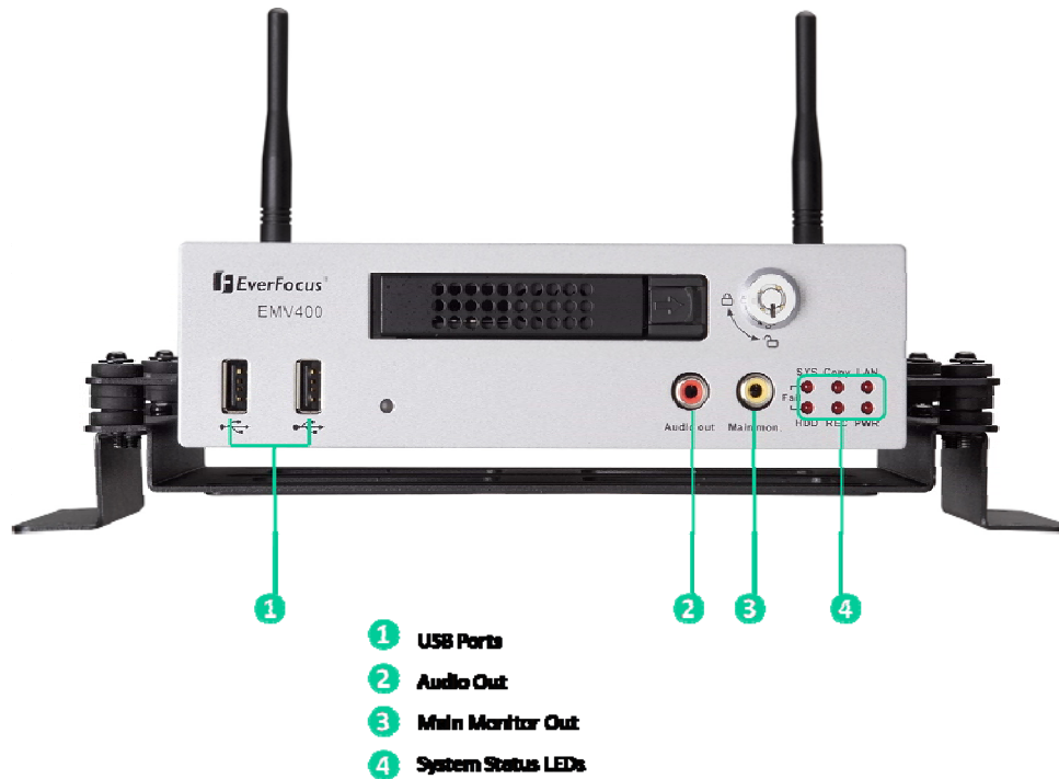
Figure 1-1 Front Panel
