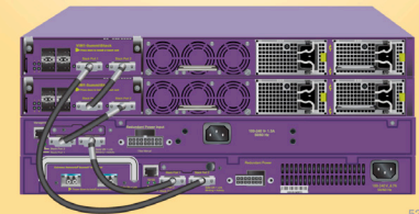
Figure 2: SummitStack Stacking Architecture
