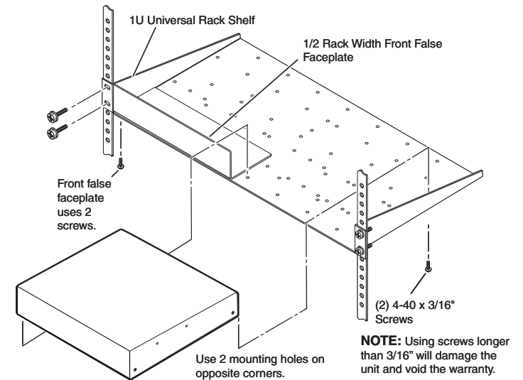
Figure 2-5 — Rack mounting the RGB 164xi
