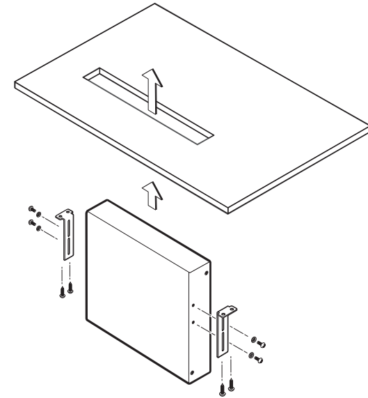
Figure 2-8 — Attaching the through desk brackets
