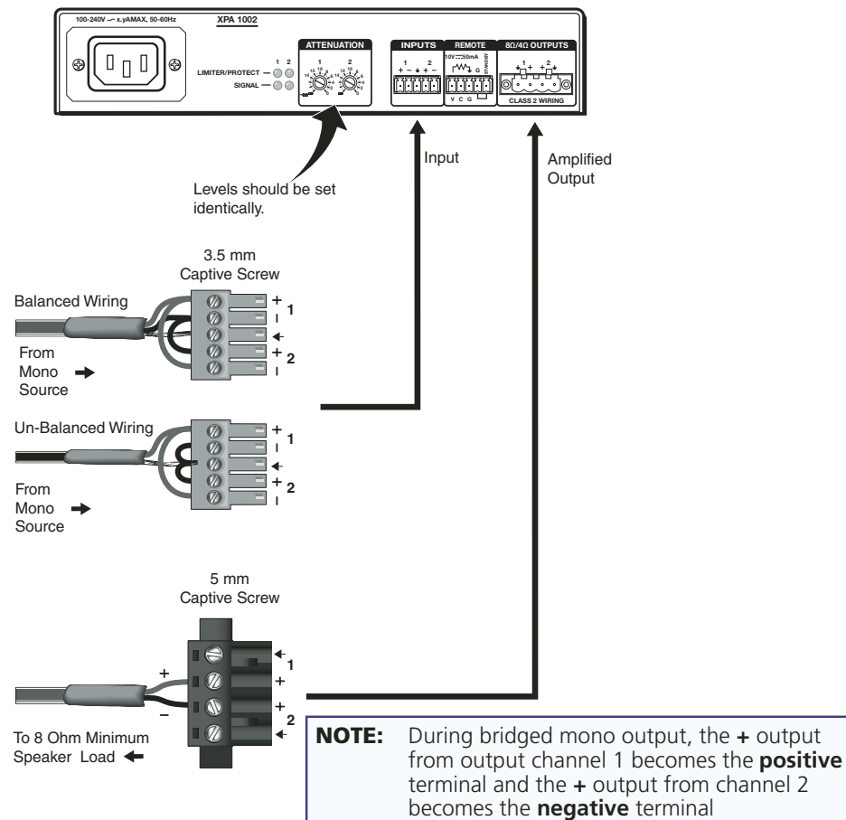
Figure 10. Bridging the Output of the XPA 1002
