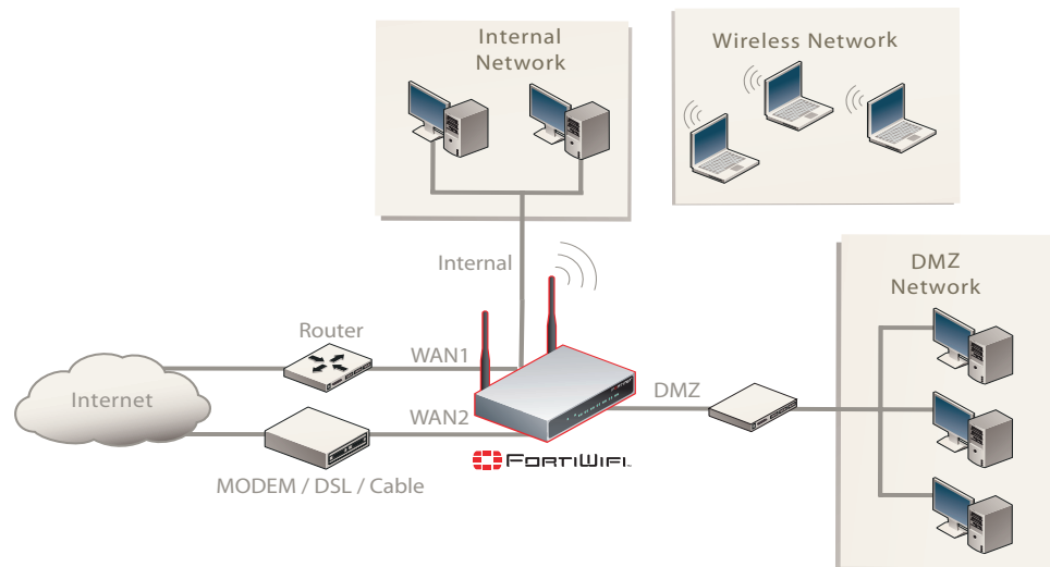
Figure 15: FortiWiFi in Access Point mode
