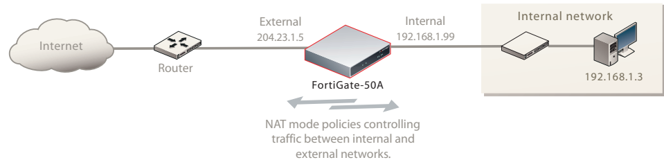
Figure 8: Example NAT/Route mode network configuration for a FortiGate-50A.
