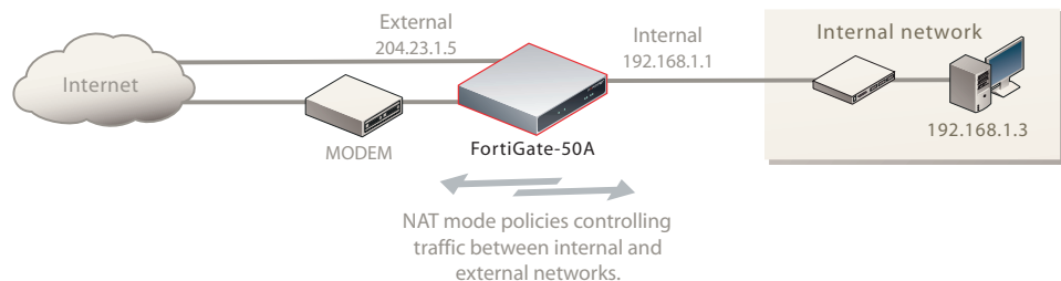
Figure 9: NAT/Route multiple internet connection configuration for a FortiGate-50A
