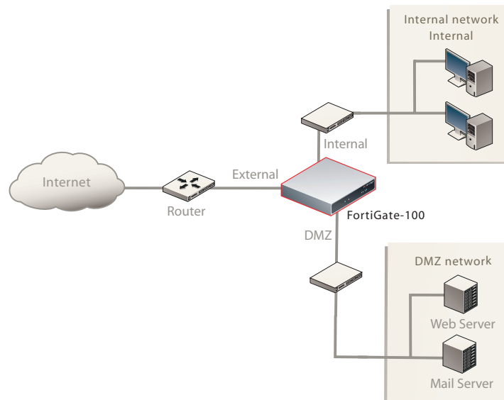
Figure 10: Example Transparent mode network configuration for a FortiGate-100
