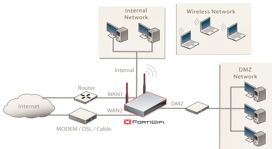
Figure 13: FortiWiFi-50B as an Access Point
