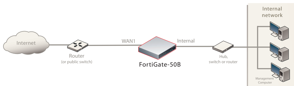
Figure 11: FortiGate-50B Transparent mode connections
