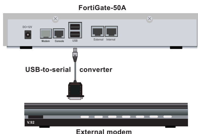
Figure 12: Example modem interface network connection
