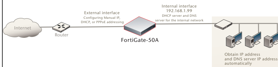
Figure 7: Quick configuration using default settings
