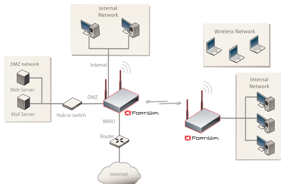
Figure 16: FortiWiFi-50B in Client mode
