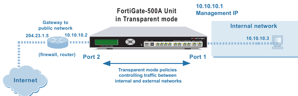
Figure 7: Example Transparent mode network configuration
