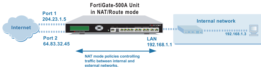
Figure 6: Example NAT/Route multiple internet connection configuration
