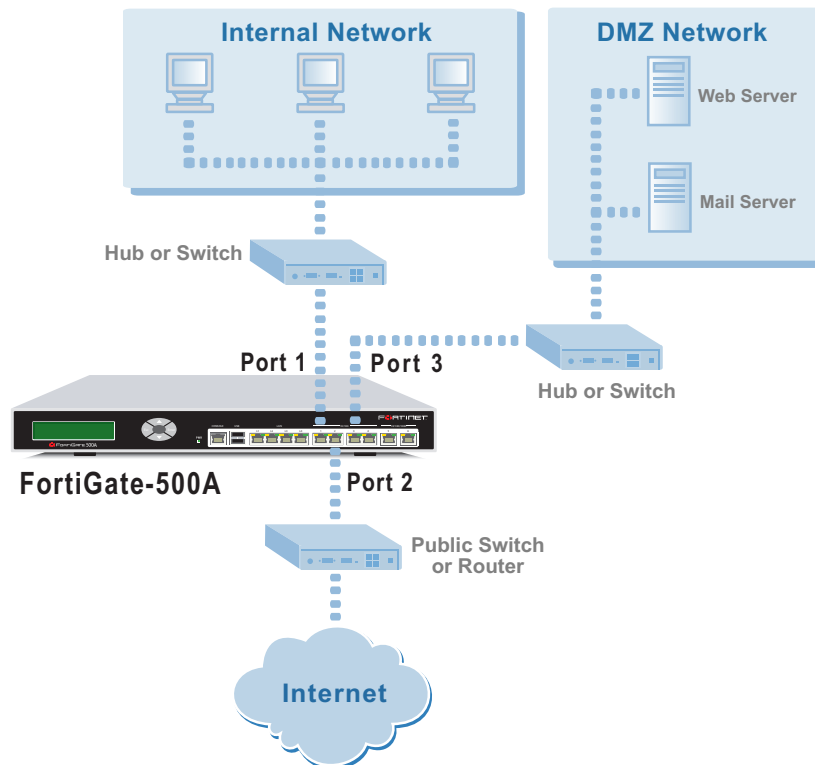
Figure 9: FortiGate-500A NAT/Route mode connections
