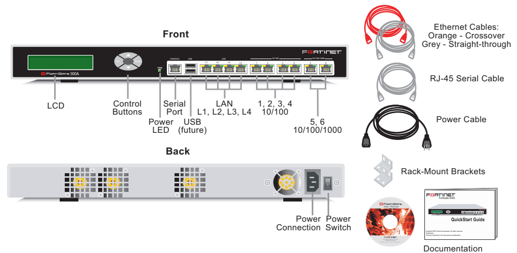
Figure 2: FortiGate-500A package contents
