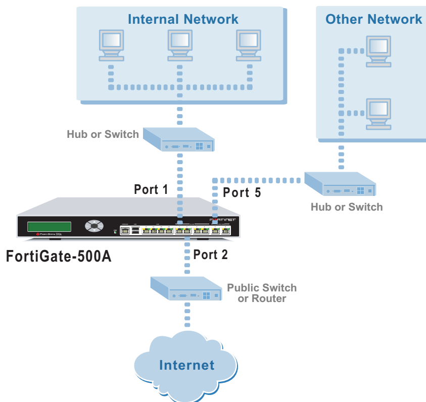
Figure 10: FortiGate-500A Transparent mode connections
