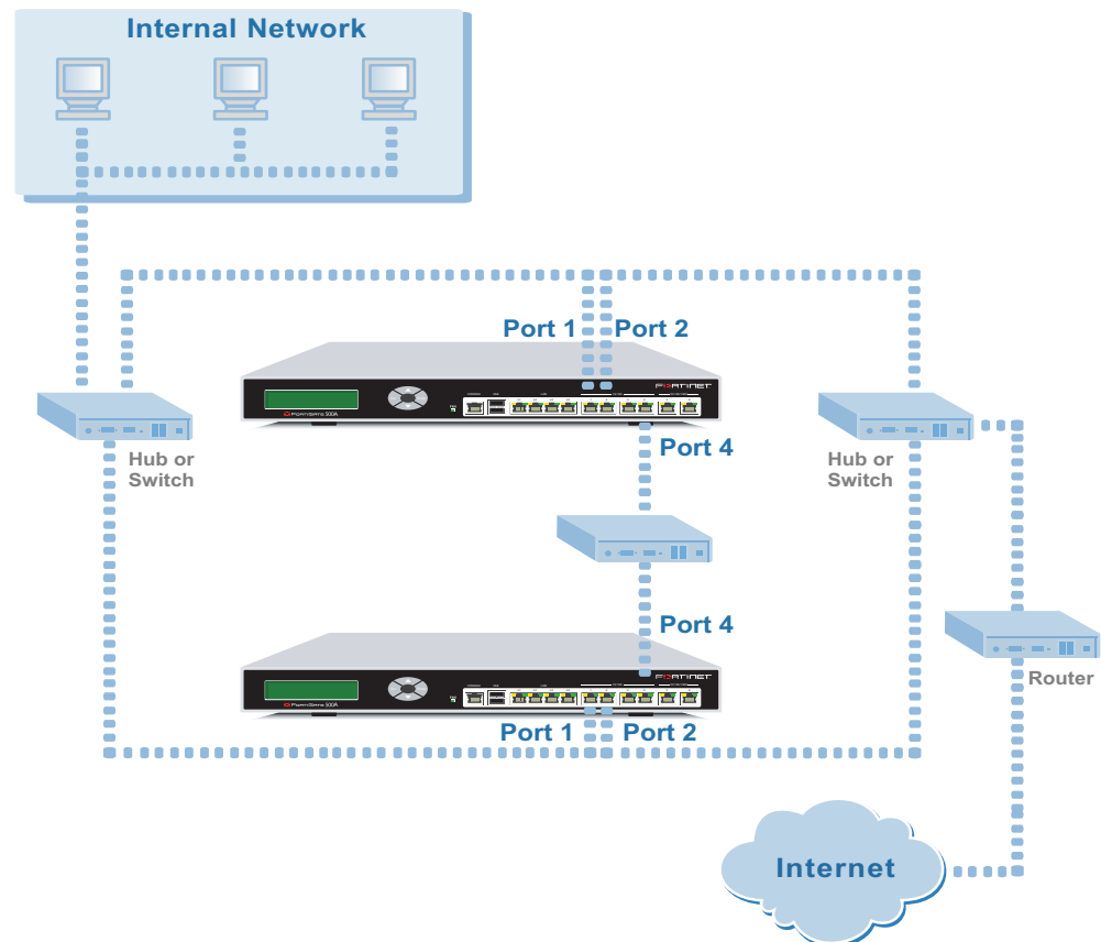
Figure 11: HA network configuration
