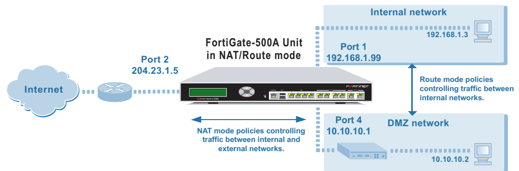
Figure 5: Example NAT/Route mode network configuration
