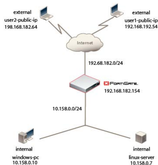
Figure 13: SSL VPN configuration for unique access permissions
