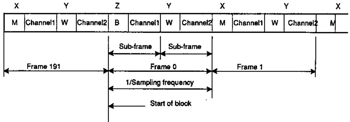
Figure 23 Frame format
