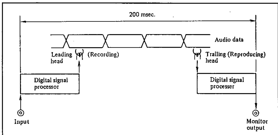
Figure 7 Confidence monitor
