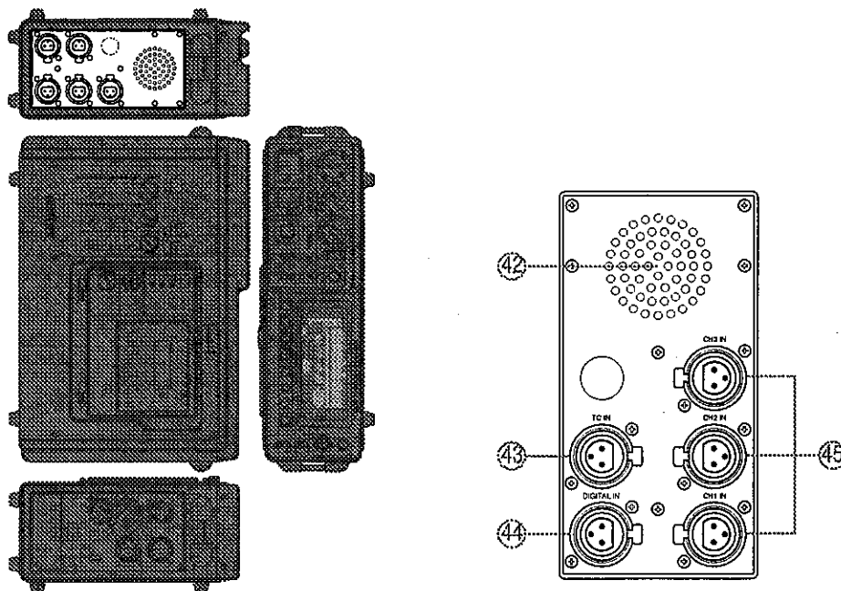
Figure 7 Input connectors
