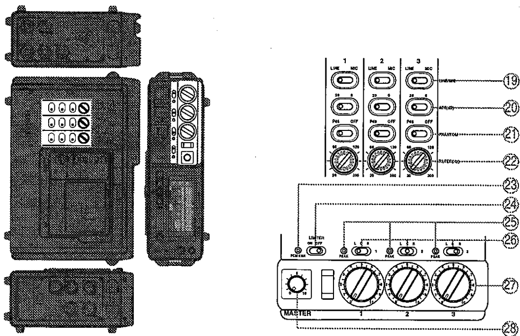
Figure 4 Mixer controls
