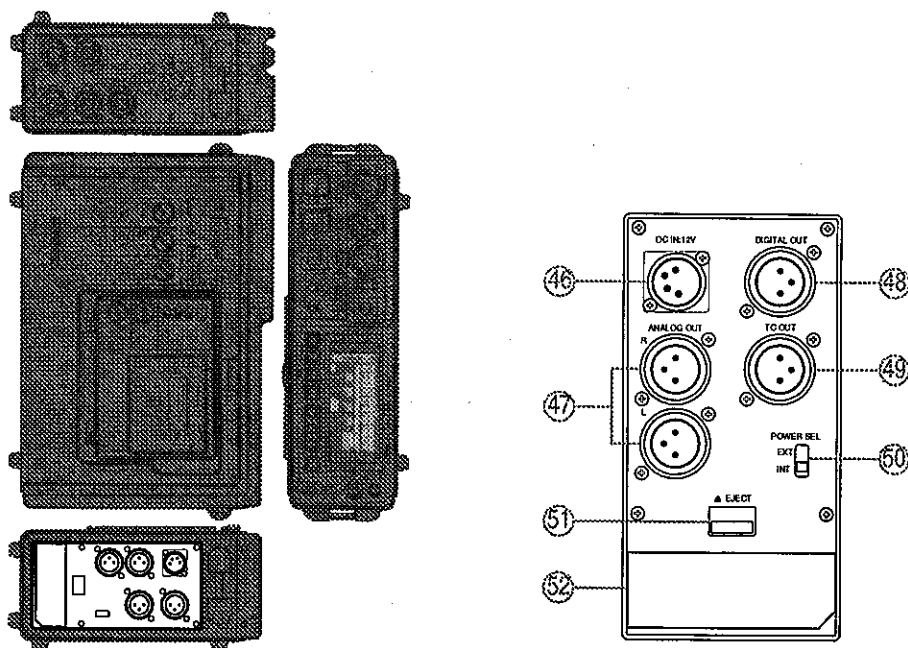
Figure 8 Output connectors
