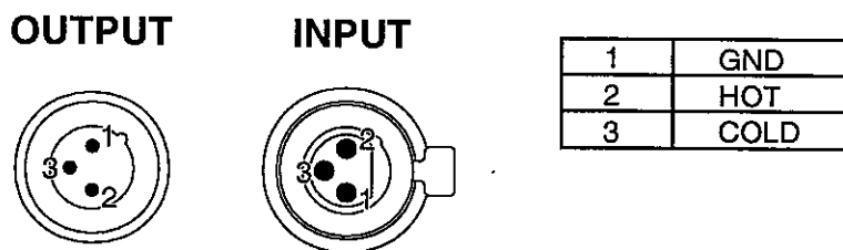
Figure 30 XLR wiring
