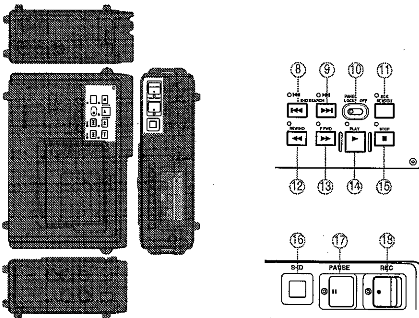
Figure 3 Transport controls
