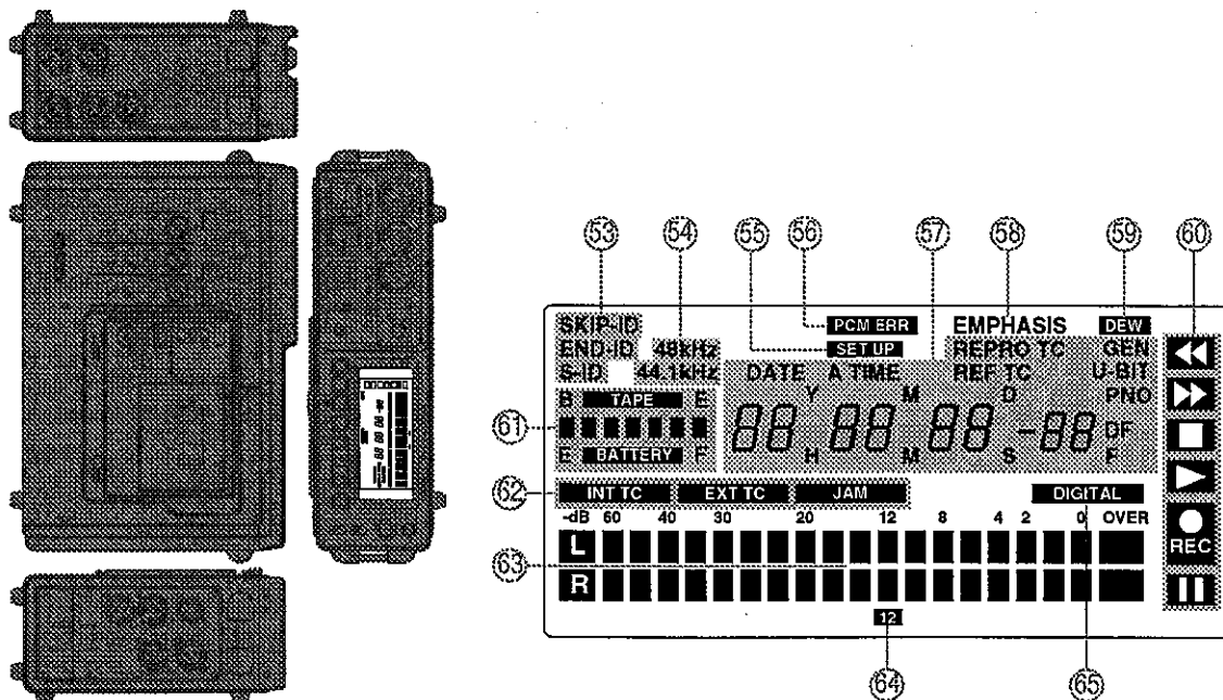
Figure 9 LCD panel
