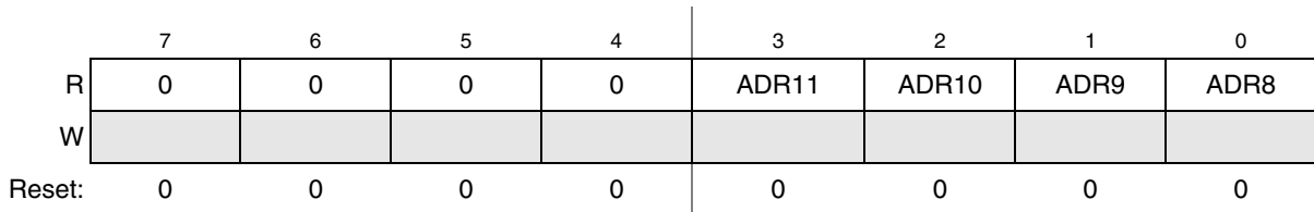
Figure 11-5. Data Result High Register (ADCRH)
