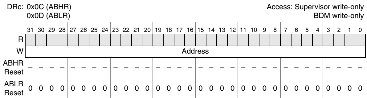
Figure 18-13. Address Breakpoint Registers (ABLR, ABHR)
