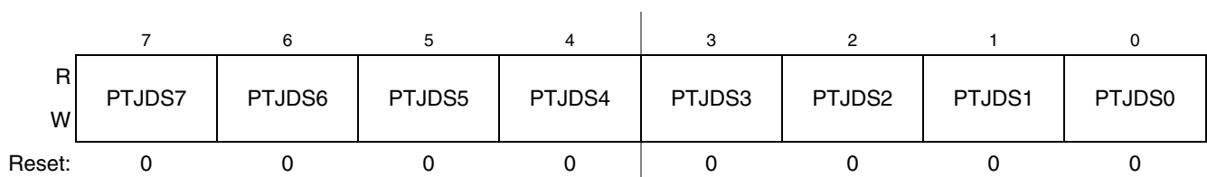
Figure 6-54. Drive Strength Selection for Port J Register (PTJDS)
