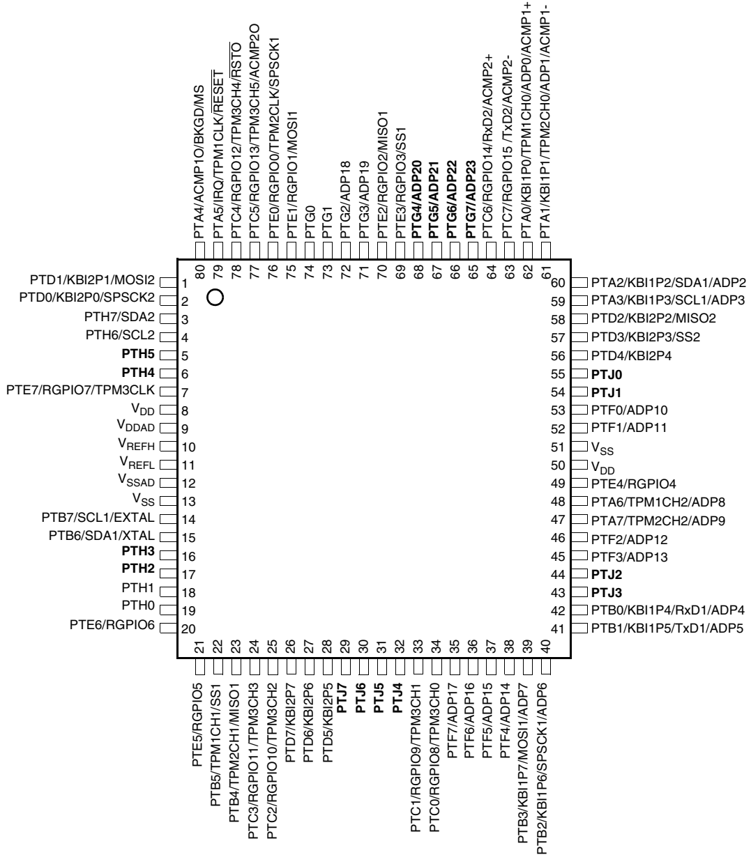
Figure 2-1. 80-Pin LQFP
