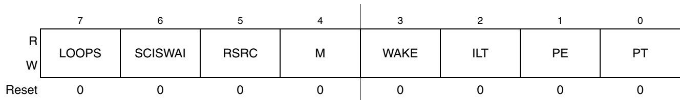
Figure 15-7. SCI Control Register 1 (SCIxC1)
