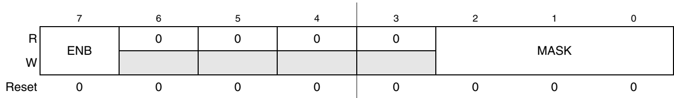
Figure 8-4. INTC_WCR Register
