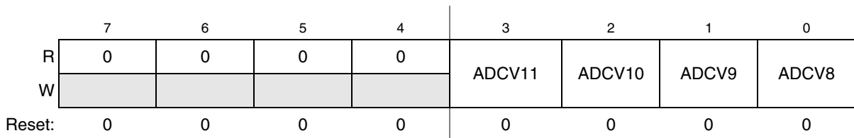
Figure 11-7. Compare Value High Register (ADCCVH)
