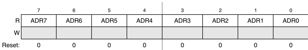
Figure 11-6. Data Result Low Register (ADCRL)
