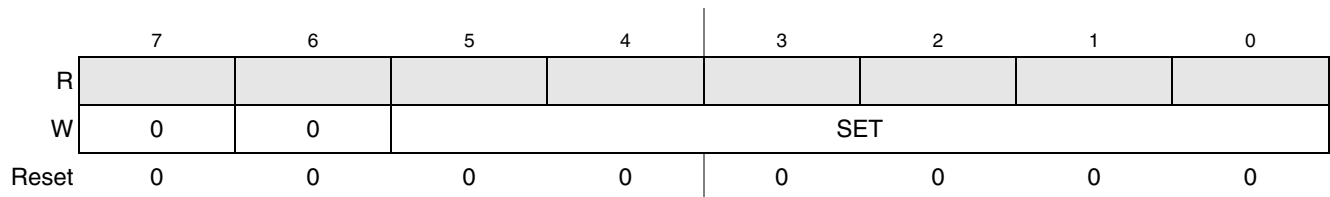
Figure 8-5. INTC_SFRC Register
