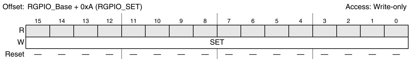
Figure 9-8. RGPIO Set Data Register (RGPIO_SET)
