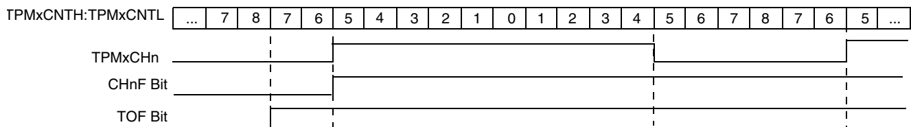
Figure 17-5. High-True Pulse of a Center-Aligned PWM
