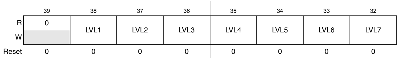
Figure 8-2. INTC_FRC Register
