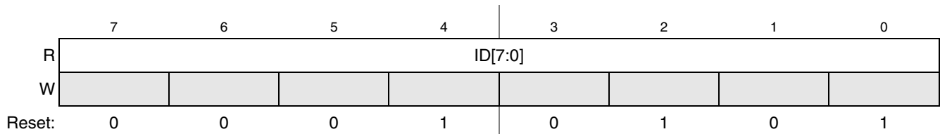
Figure 5-6. System Device Identification Register Low (SDIDL)
