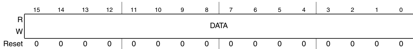
Figure 9-5. RGPIO Data Register (RGPIO_DATA)
