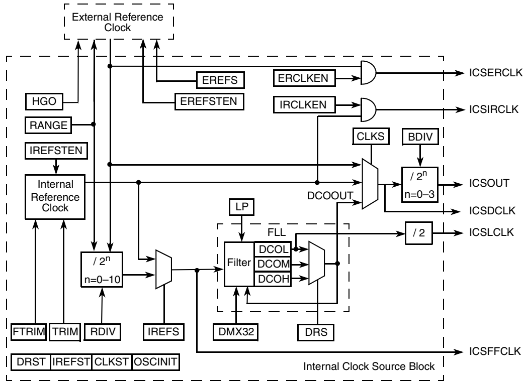
Figure 12-2. Internal Clock Source (ICS) Block Diagram
