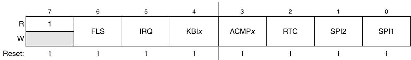
Figure 5-11. System Clock Gating Control 2 Register (SCGC2)
