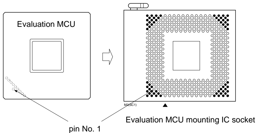
Figure 4.3-2 Mounting Position
