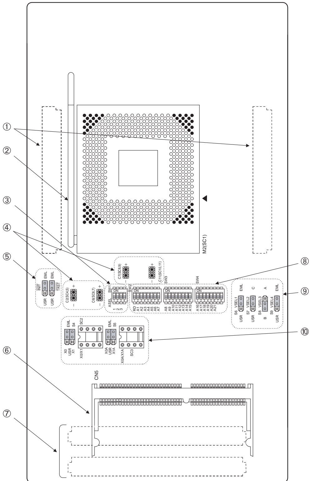
Figure 2.2-1 External View
