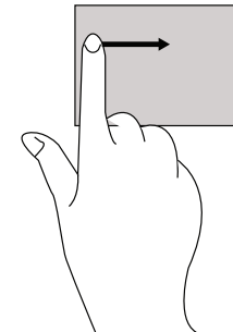
Figure 31. Dernière application
