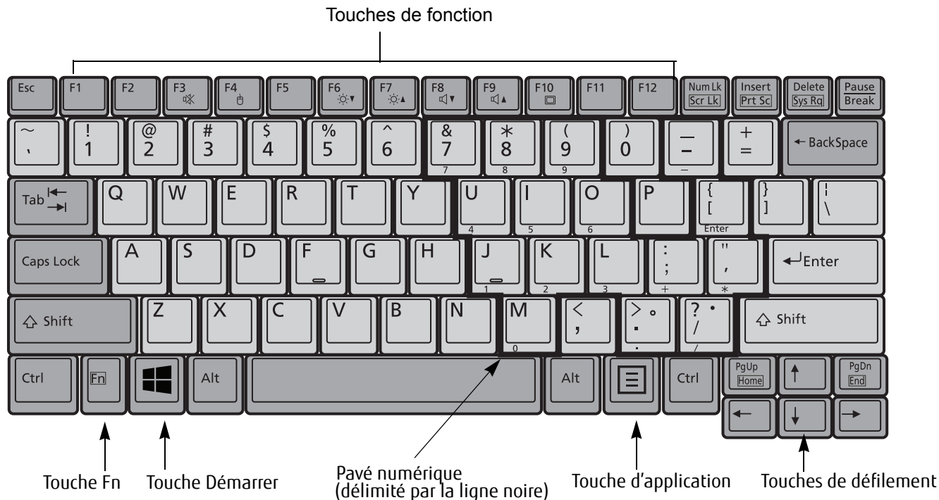
Figure 12. Clavier
