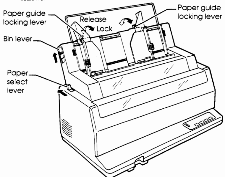
Preparing the cut sheet feeder
