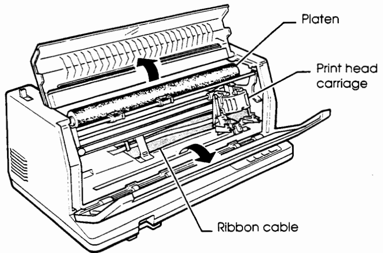
Printer interior
