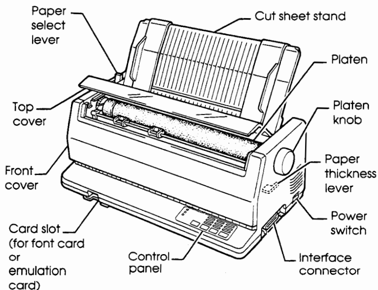
Front and side view of printer
