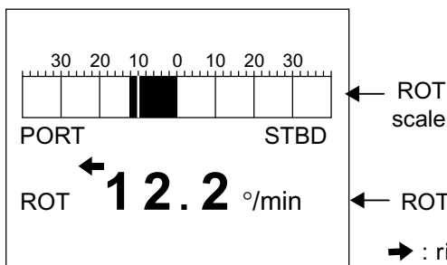
ROT (Rate Of Turn display)
