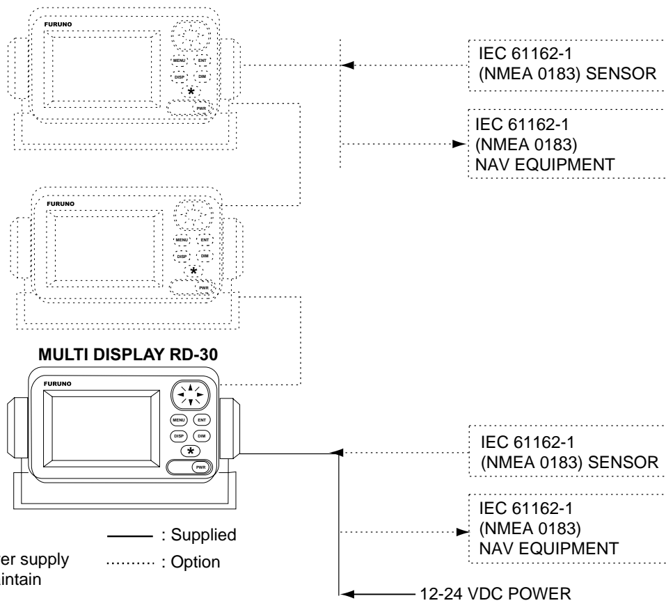
Example of multiple display unit connection
