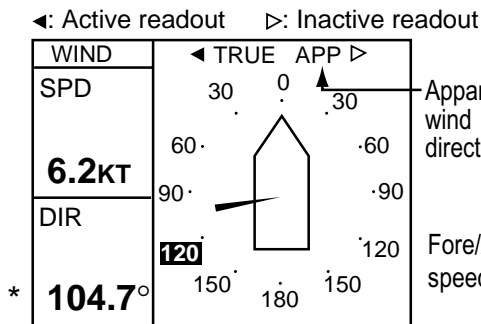
Wind graphic display
