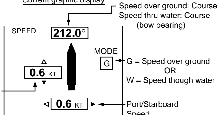
Speed graphic display (SOG or STW)
