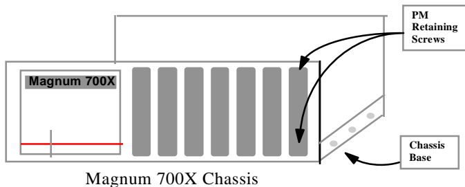
Figure 3.3c: Front Panel View - PM Retaining Screws
