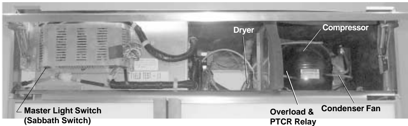
Figure 1 - Machine Compartment
