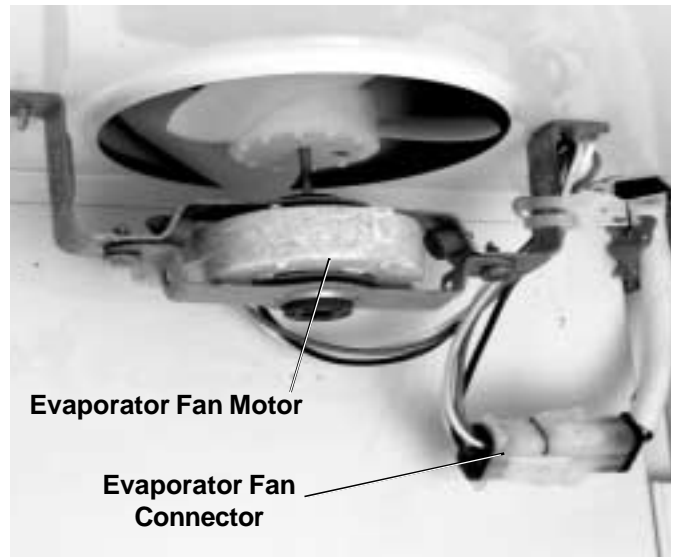
Figure 4 - Evaporator Fan
