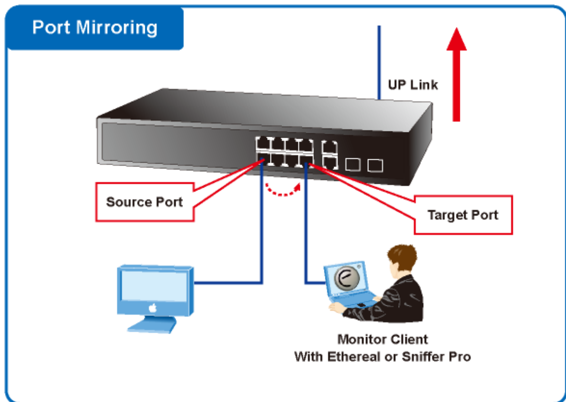
Figure 44: Port Mirror application
