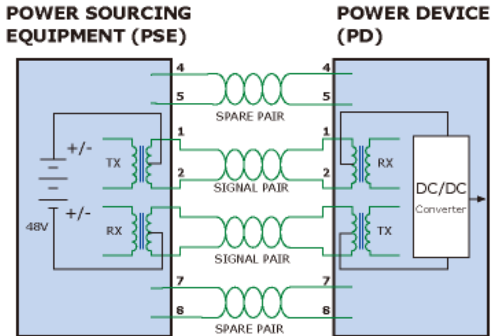
Figure 100: Power Supplied over the Data Pins
