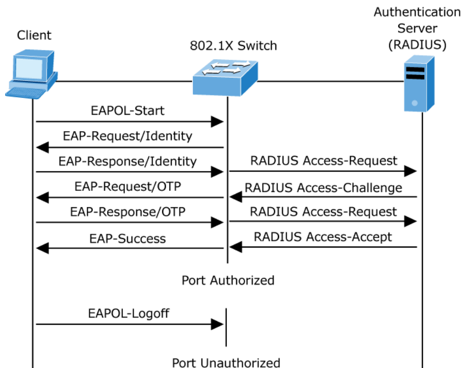
Figure 87: EAP message exchange
