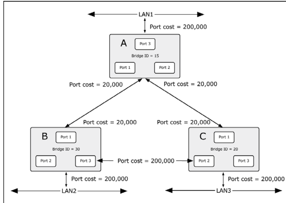
Figure 59: Before Applying the STA Rules
