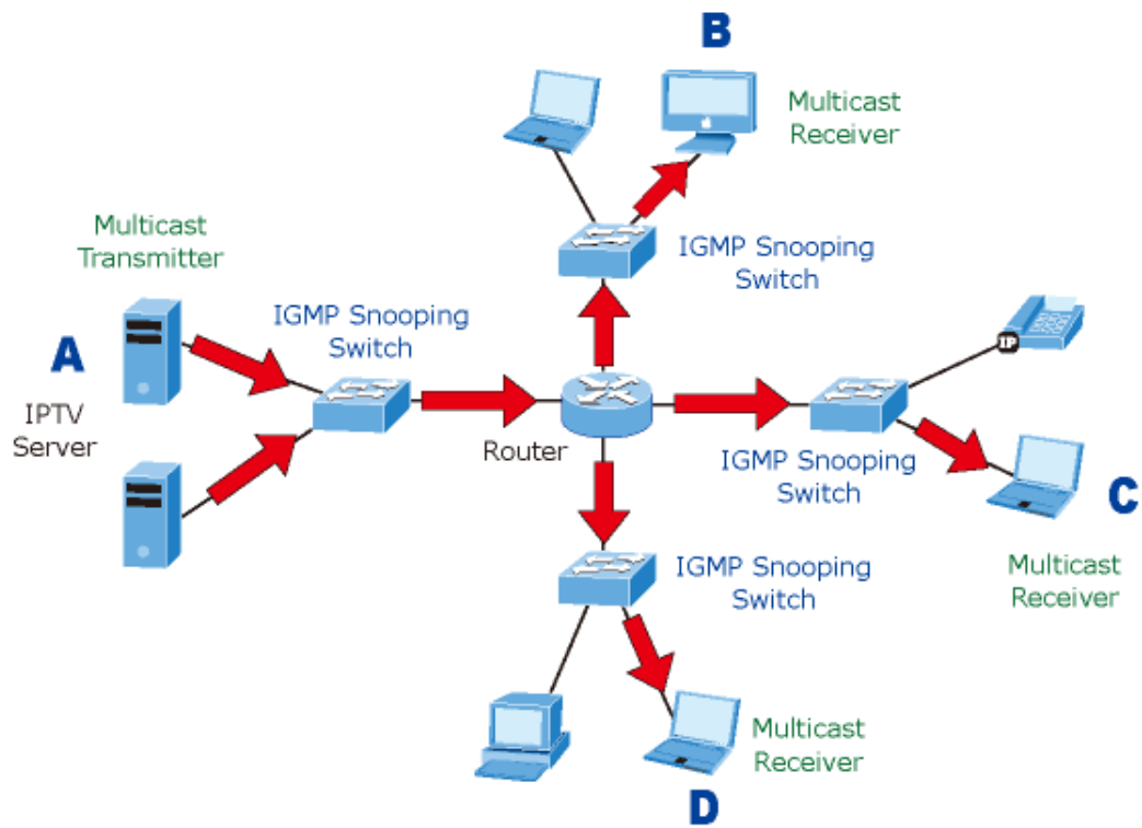
Figure 76: IGMP Snooping multicast stream control
