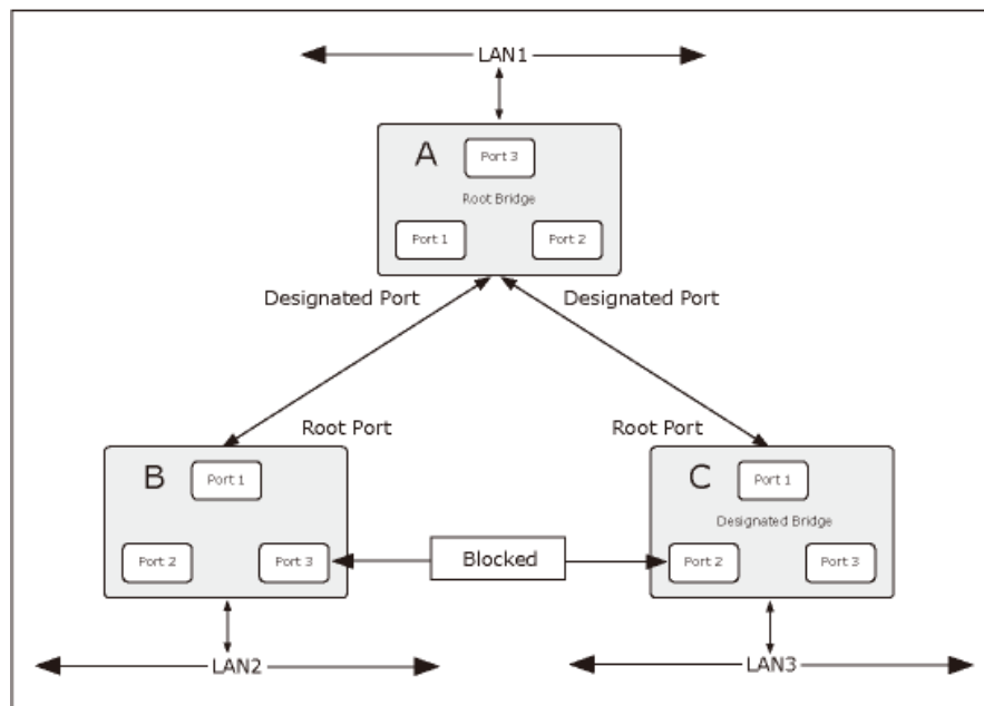
Figure 60: After Applying the STA Rules
