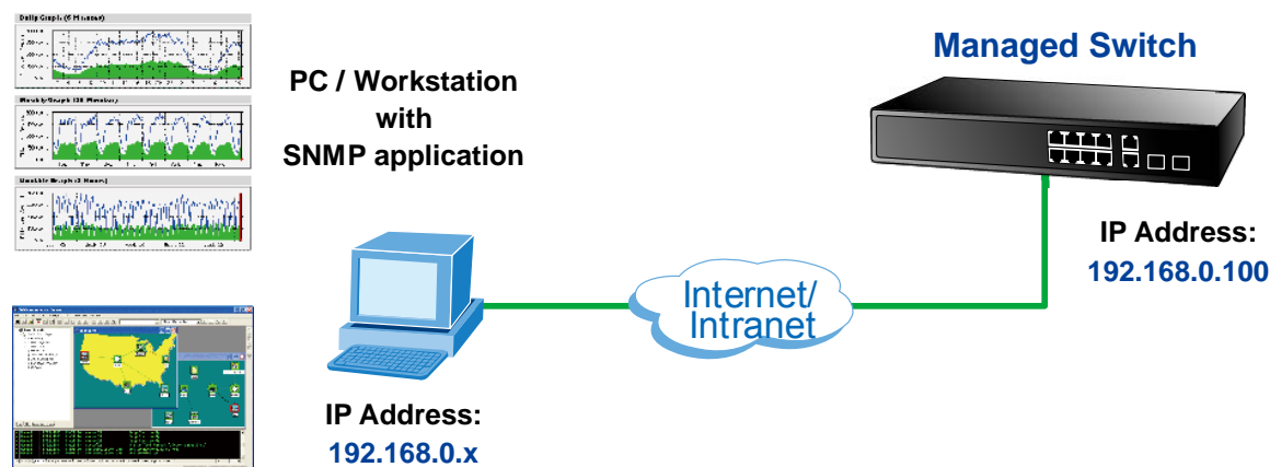
Figure 13: SNMP Management
