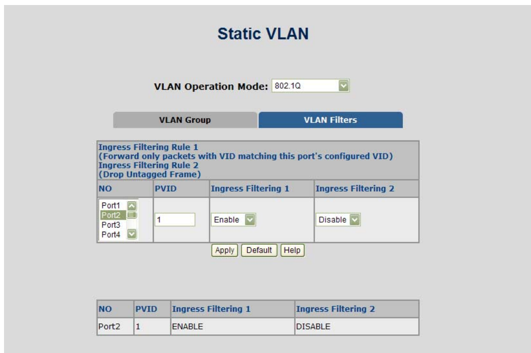
Figure 53: 802.1Q Ingress filter interface
