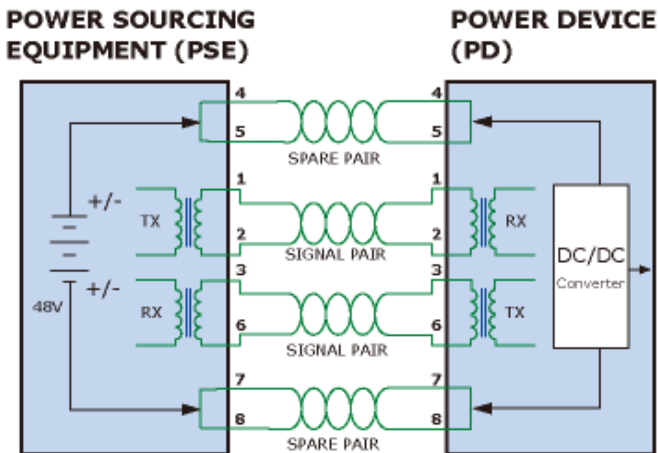
Figure 99: Power Supplied over the Spare Pins
