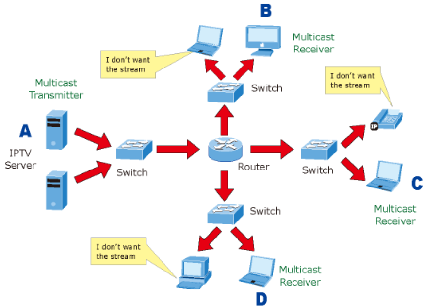
Figure 75: Multicast flooding
