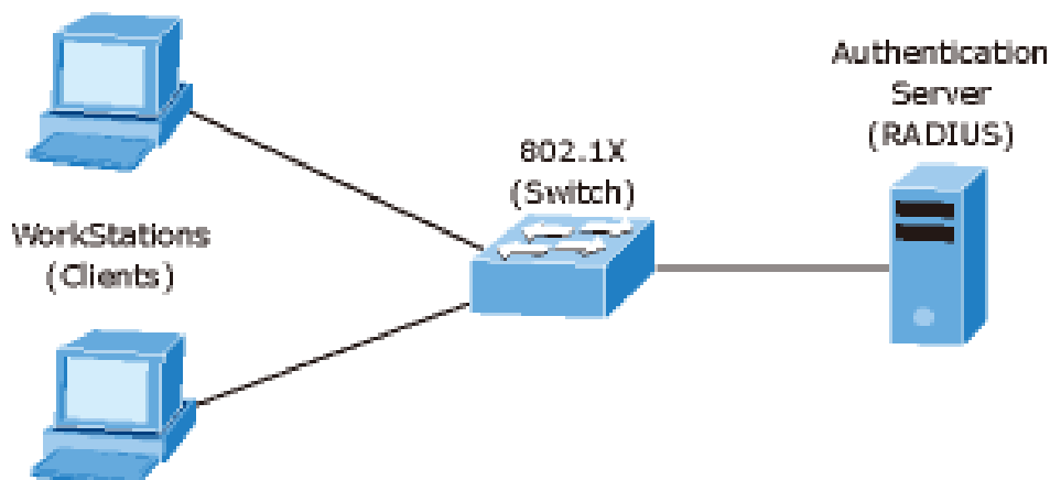
Figure 86: 802.1x device role
