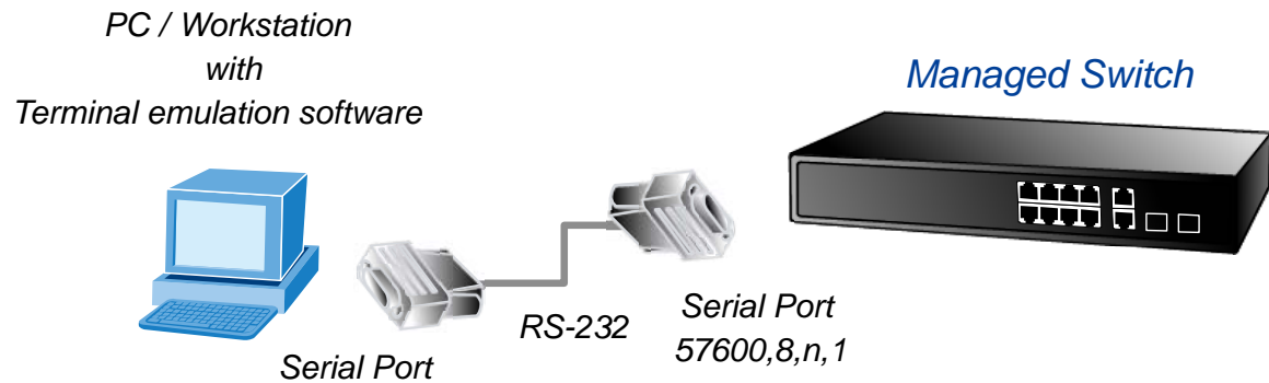
Figure 14: PC connected to Switch with RS-232 serial cable
