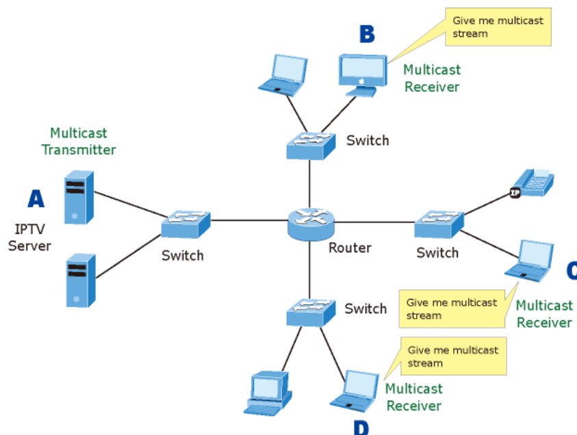
Figure 74: Multicast Service
