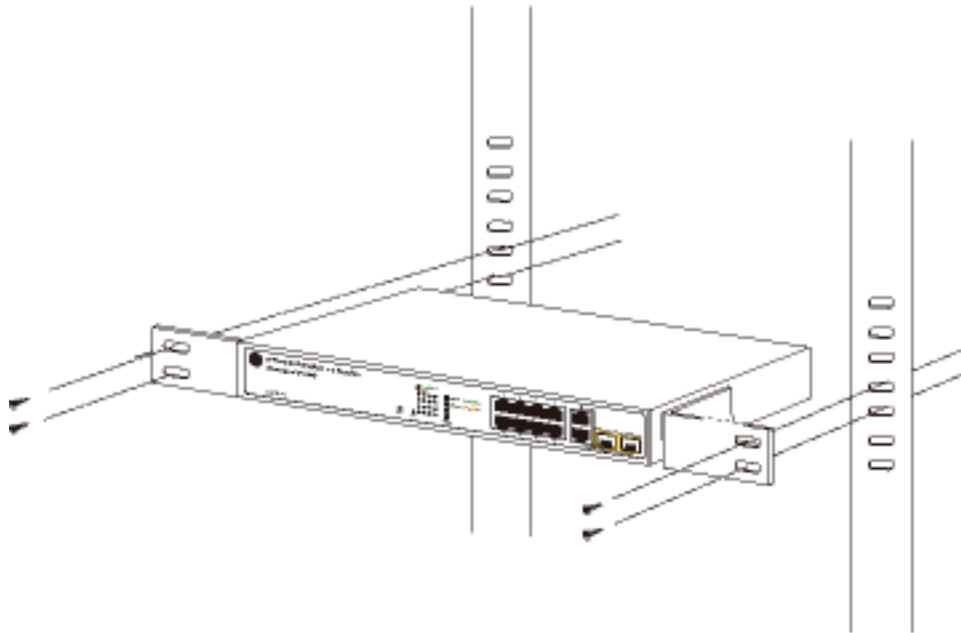
Figure 7: Mounting the GE-DS-82 in a rack
