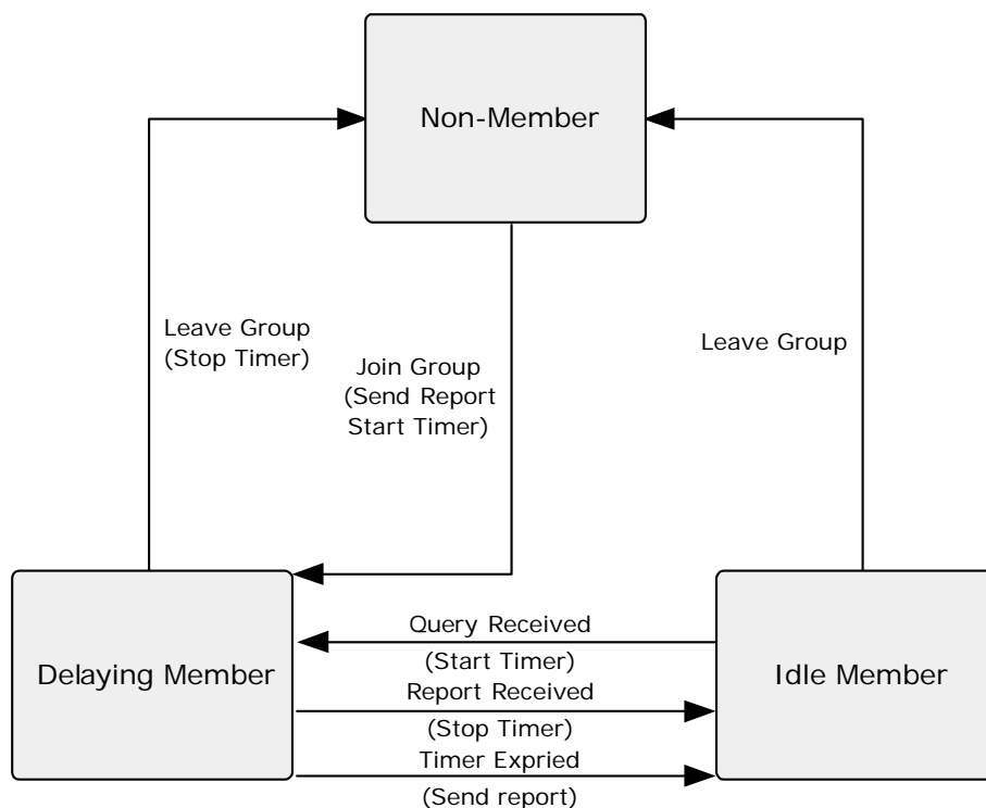
Figure 77: IGMP State Transitions
