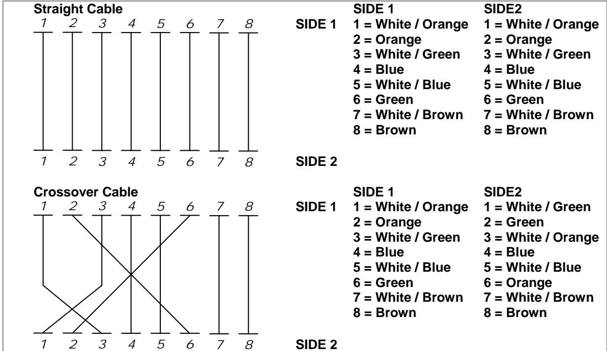
Figure 101: Straight-Through and Crossover Cable
