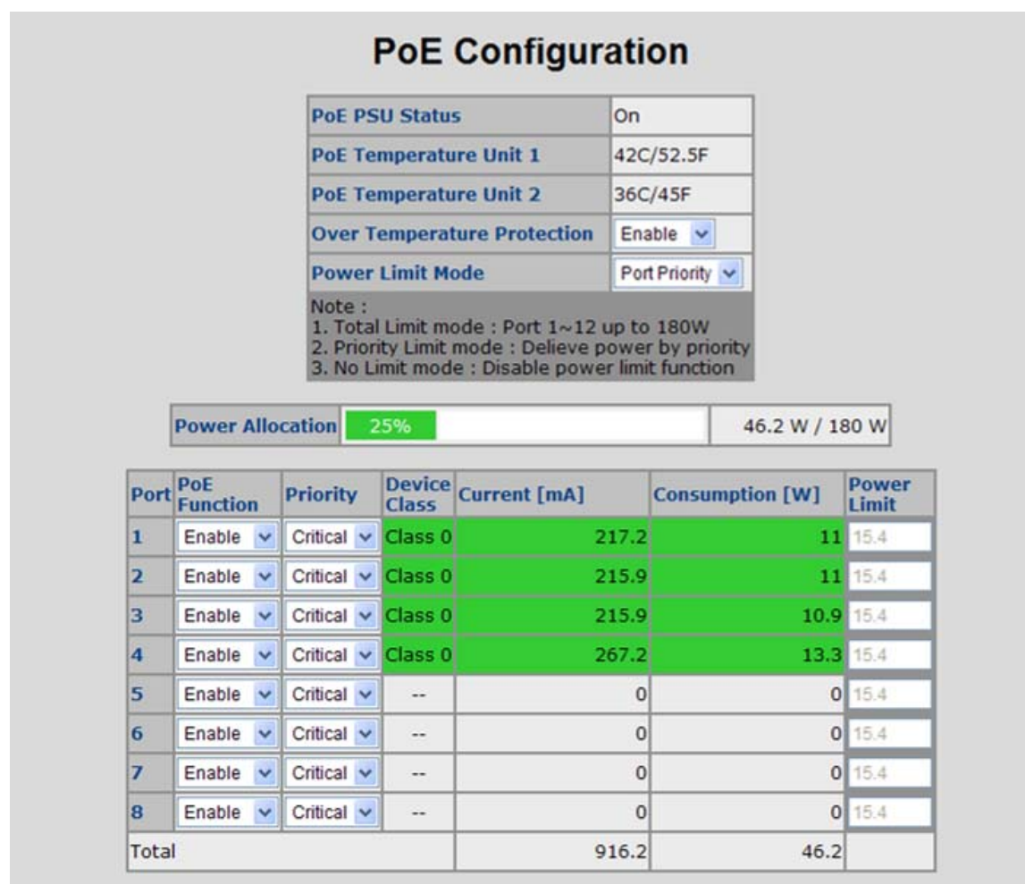
Figure 92: PoE Configuration
