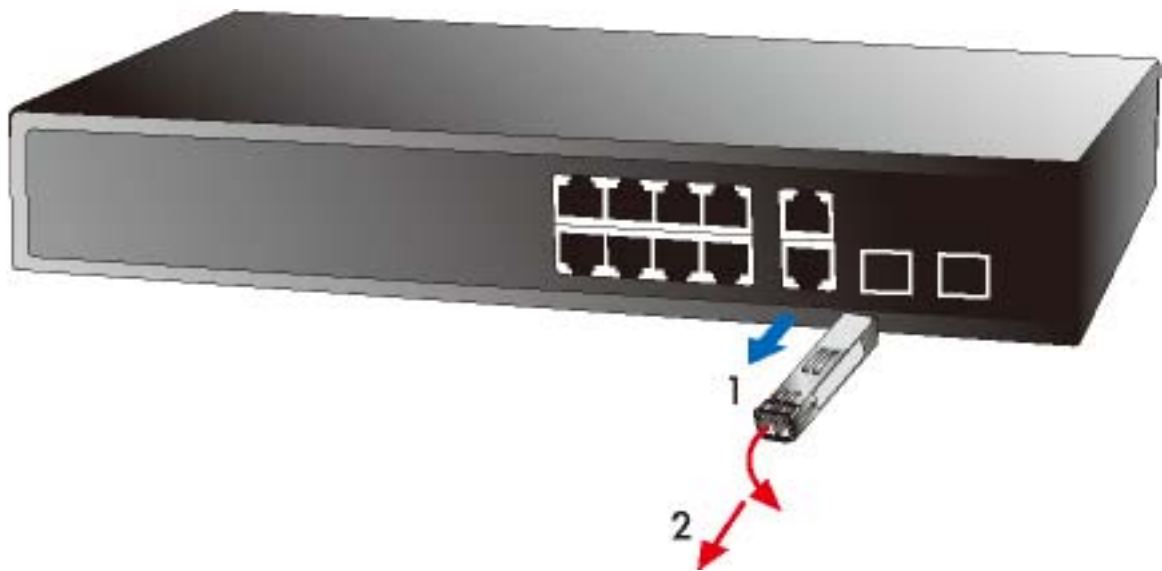
Figure 9: Pulling out the SFP transceiver
