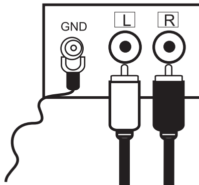
Figure G - Connect the included RCA cable and ground spade to the respective RCA jacks and ground terminal found on the rear panel of your turntable.
