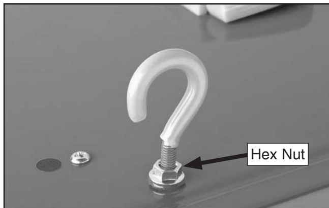
Figure 10. Machine hook partially threaded to adjust the hanging length.
