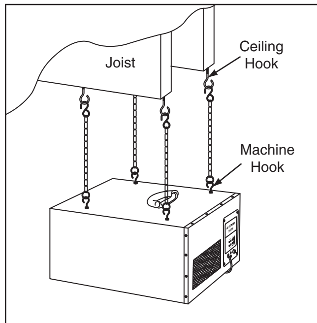
Figure 11. Air filter mounted to the joists.
