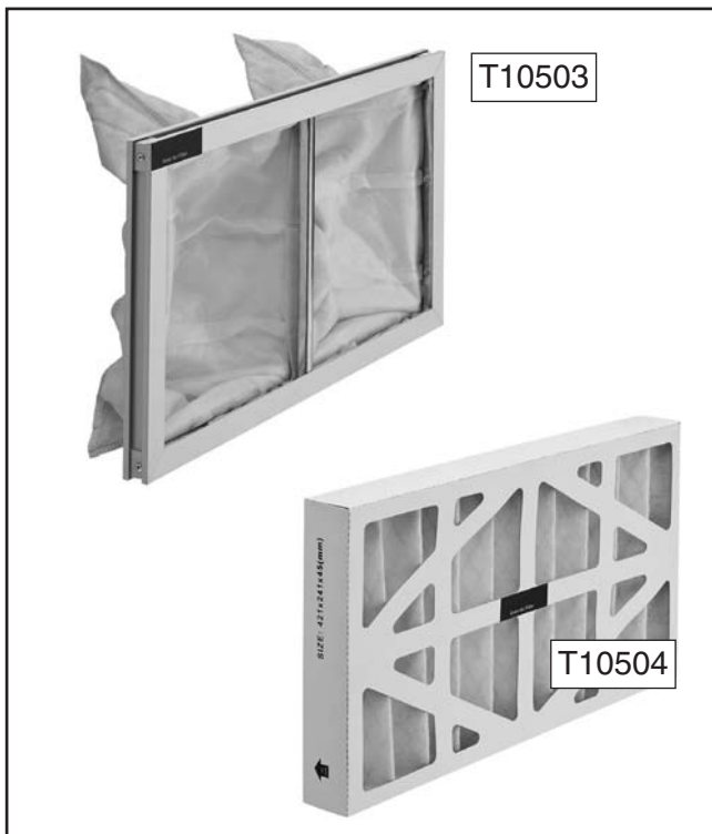
Figure 12. Model T10503 inner filter and Model T10504 outer filter for Model G0738 air filter.
