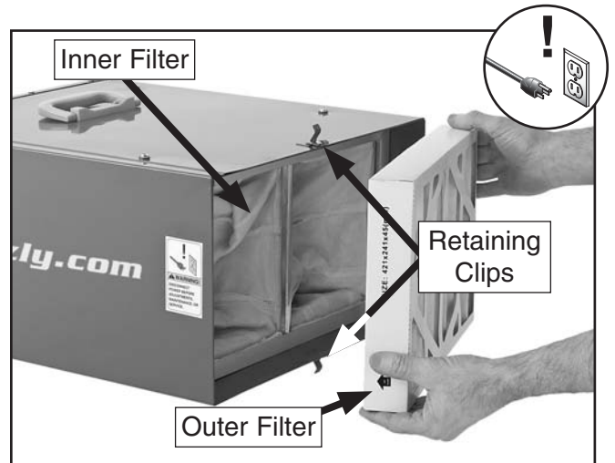
Figure 15. Filters exposed for cleaning.
