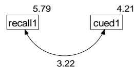
Example 10: Model A Simultaneous analysis of several groups Attig (1983) young subjects Unstandardized estimates
