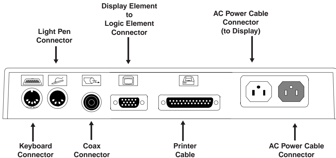
Figure 2-1. 1483 Receptacle Connectors
