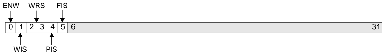
Figure 6-6. Timer Status Register (TSR)
