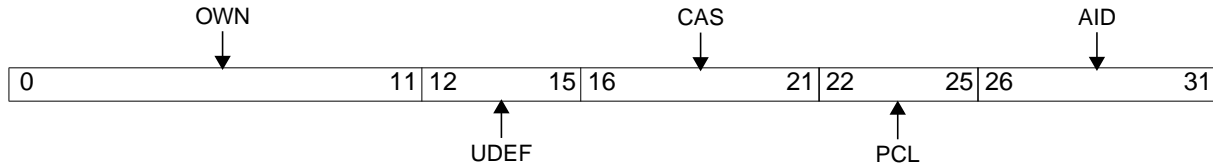
Figure 10-22. Processor Version Register (PVR)
