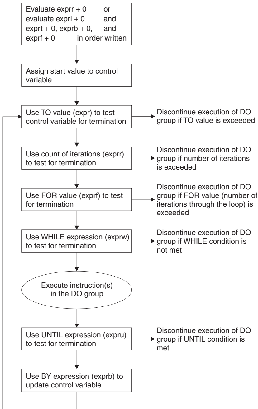
Figure 49. Concept of a DO Loop
