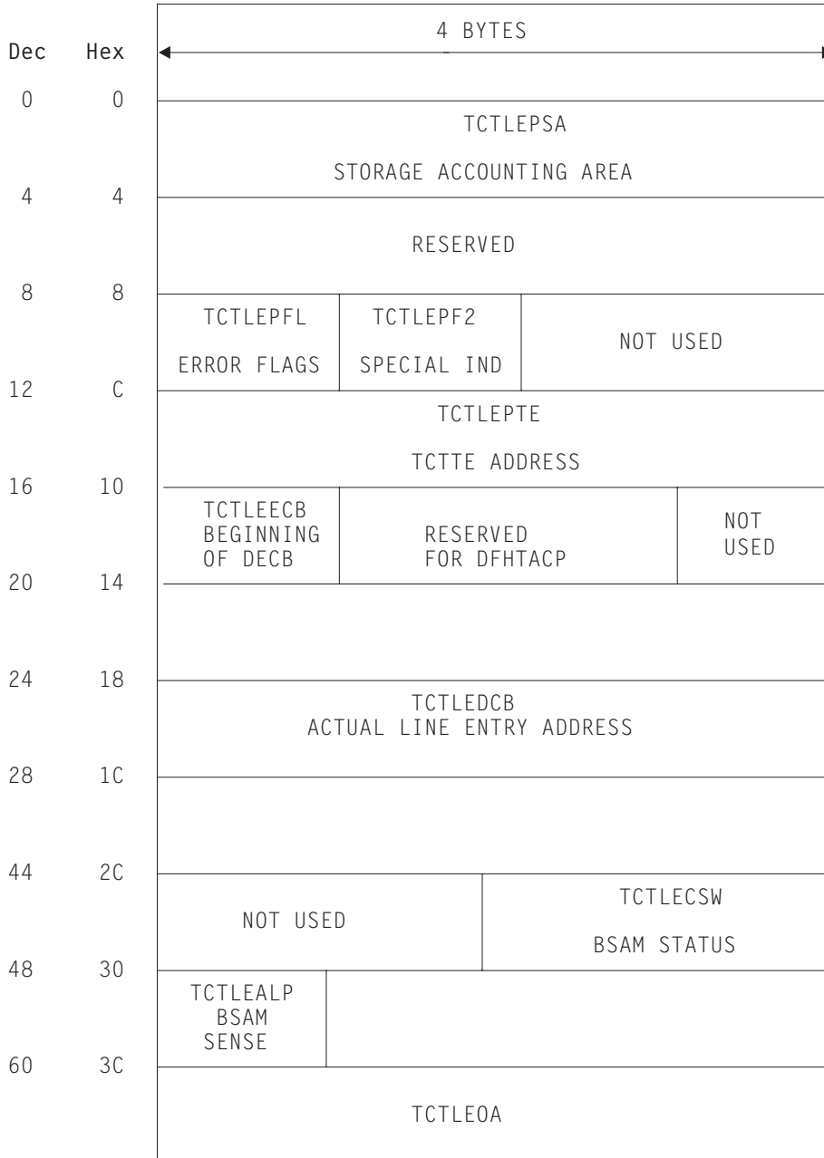
Figure 26. Format description of the TACLE DSECT (part 1)
