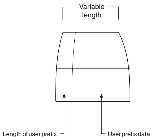
Figure 96. Format of the user prefix
