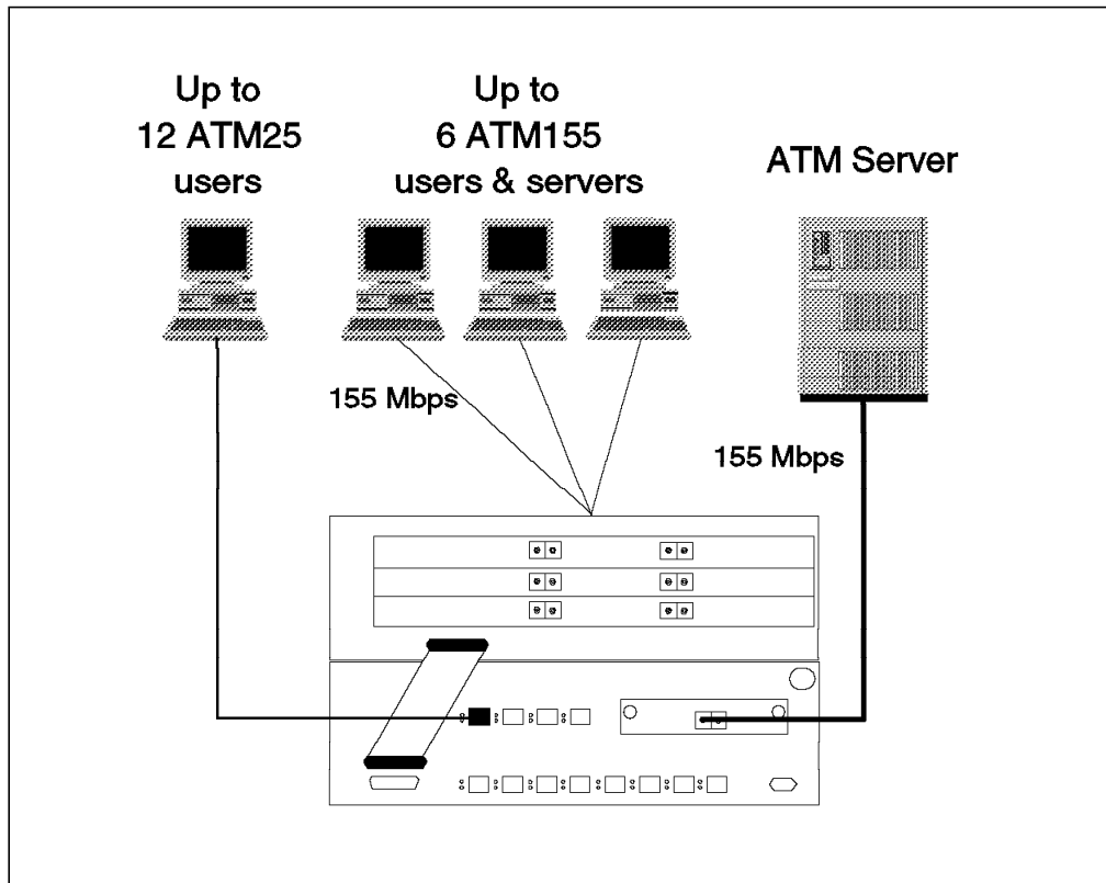
Figure 15. ATM 2-Port 155 Mbps Flexible Media Module High-Performance Workgroup
