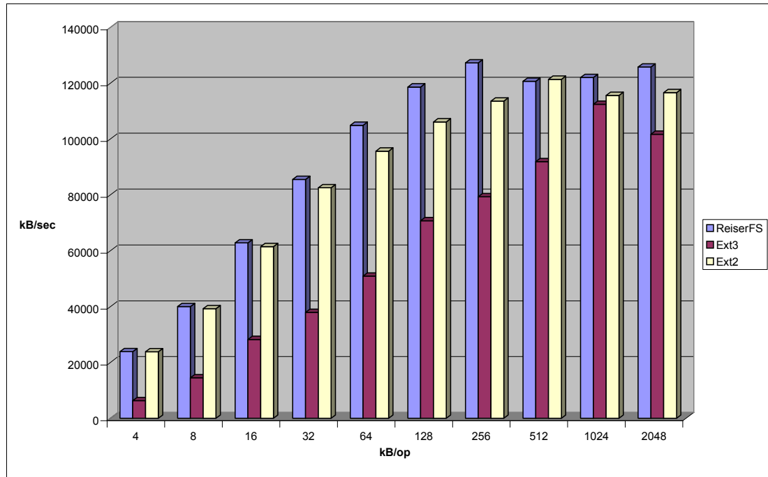
Figure 4-12 Random write throughput comparison between Ext3 and ReiserFS (asynchronous)
