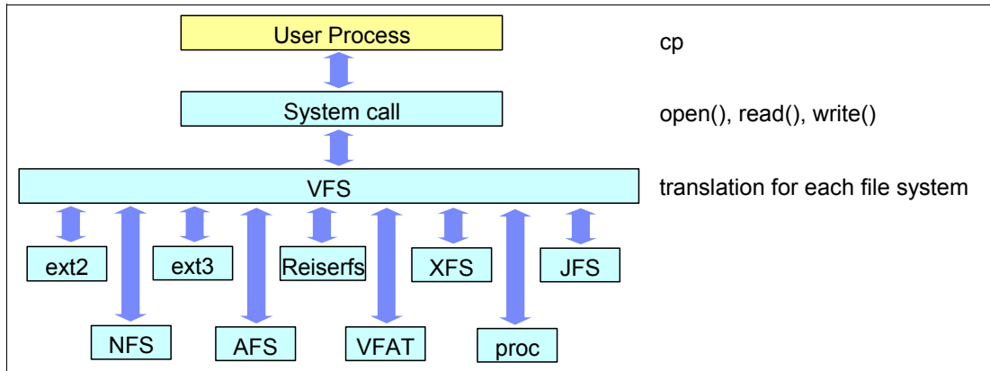
Figure 1-14 VFS concept
