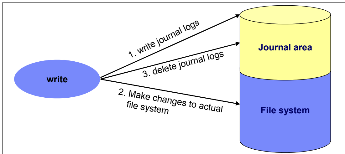
Figure 1-15 Journaling concept
