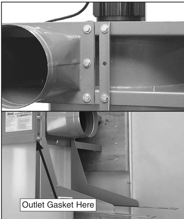
Figure 18. Model G0441 outlet port and filter L-braces installed.
