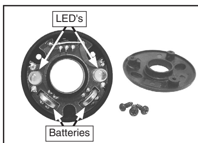
Figure 6. LED light attachment components.
