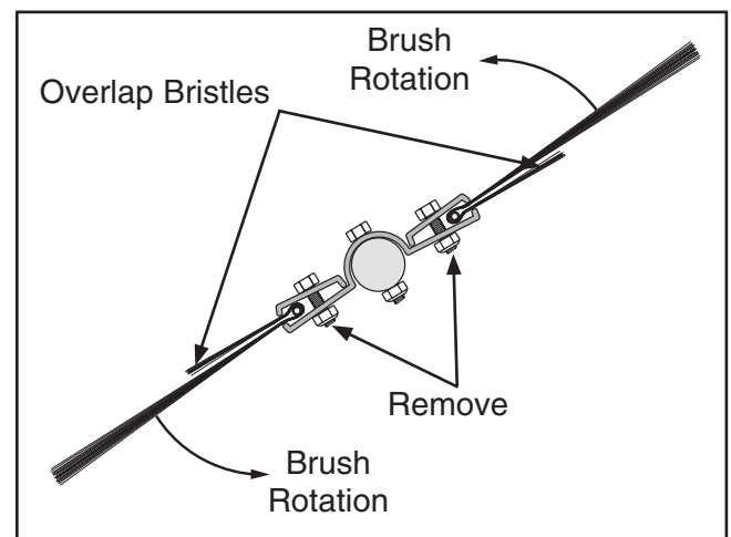
Figure 26. Brush assembly (end view).
