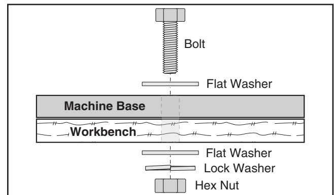
Figure 4. Through-mount method.
