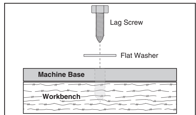
Figure 5. Direct-mount method.
