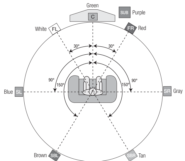
Figure 15 – Speaker Placement (7.1-Channel System)
