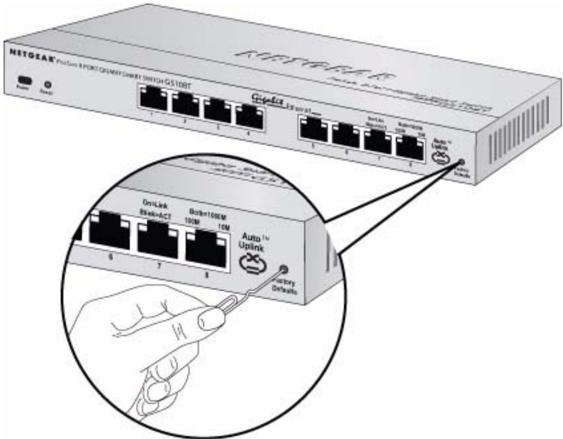
Figure 2-4 Restore Factory Defaults Button of the GS108T Gigabit Smart Switch
