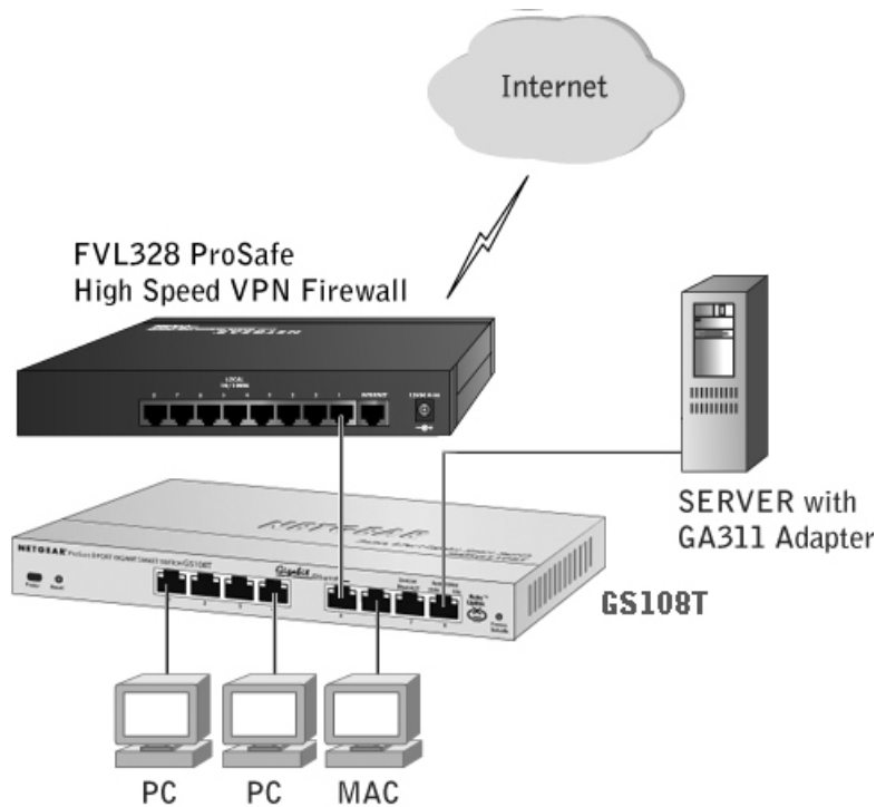
Figure 3-1 Example of Desktop Switching
