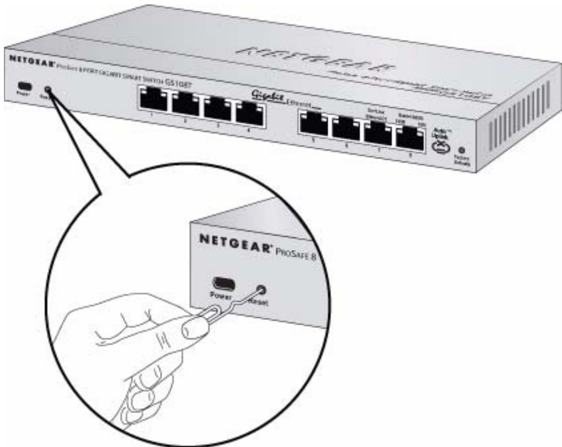
Figure 2-3 Reset Button of the GS108T Gigabit Smart Switch
