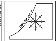
Fig 6 — Air Conditioning Process * (See Above)
